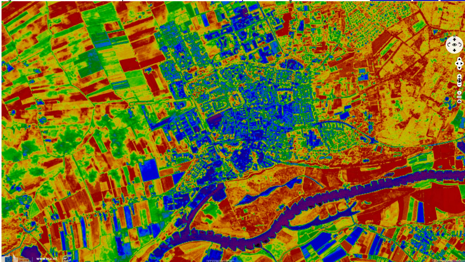
Fig. 2 - S2 MSI - NDVI with colour map - Water bodies & artificial land clearly differ from vegetated land.
