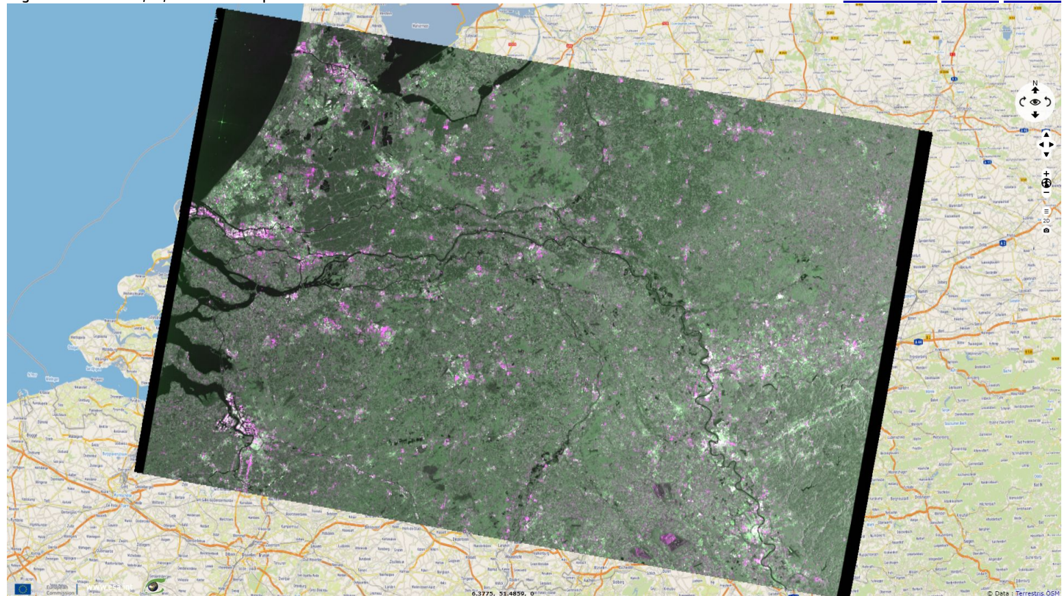
Fig. 4 - S1 IW - vv,vh,ndi(vh,vv) colour composite - Wageningen hosts Tropenbos International headquarters.
