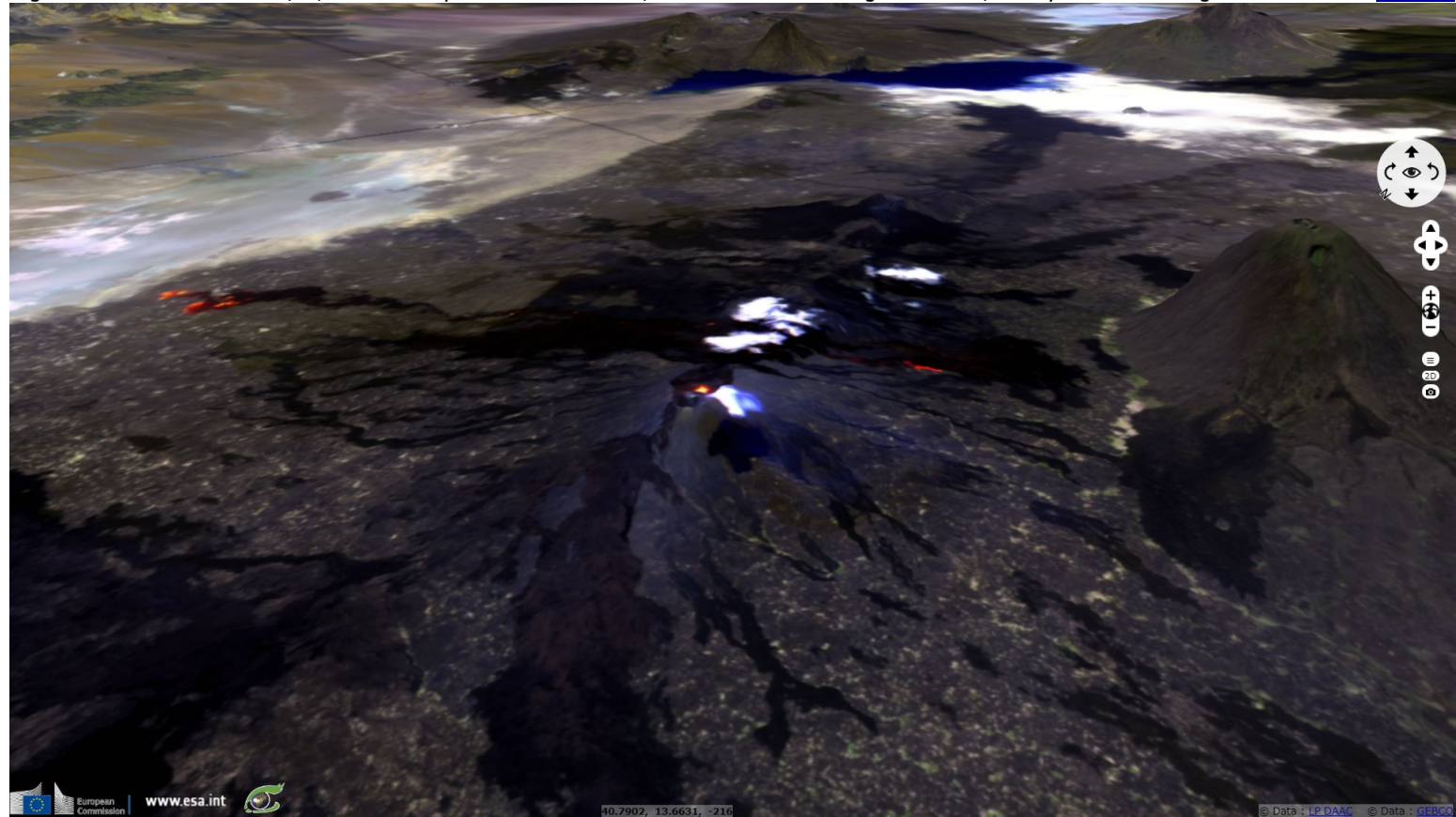
Fig. 4 - S2 (10.03.2018) - 12,11,4 colour composite - The two lava lakes has disappeared after the eruption on 16 december 2018.
