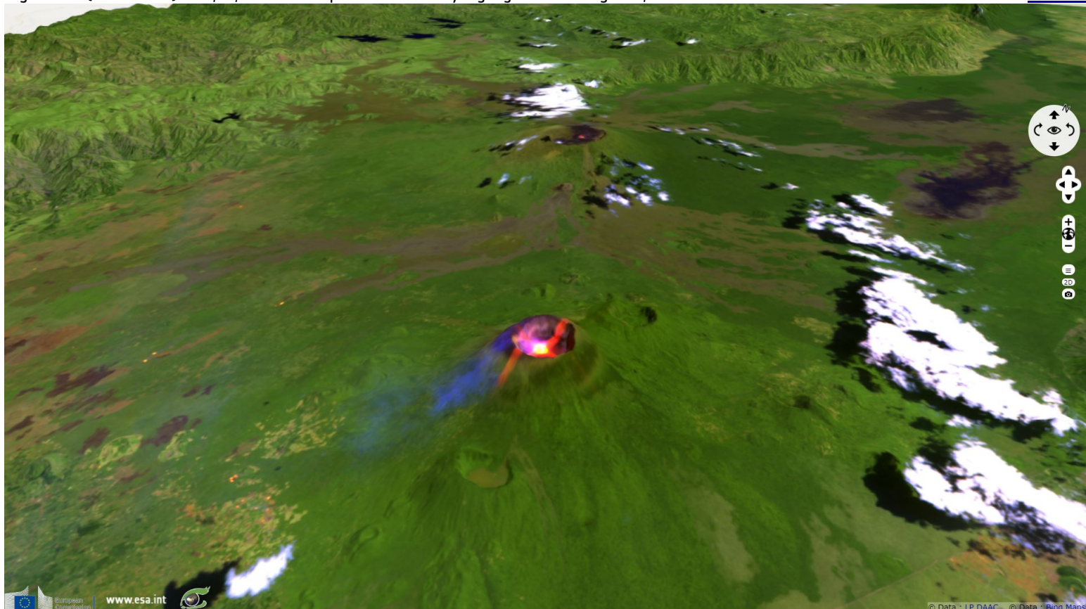
Fig. 2 - S2 (16.08.2019) - 12,11,4 colour composite - Mount Nyiragongo culminating at 3,470m shows a beautiful lava lake on its center.
