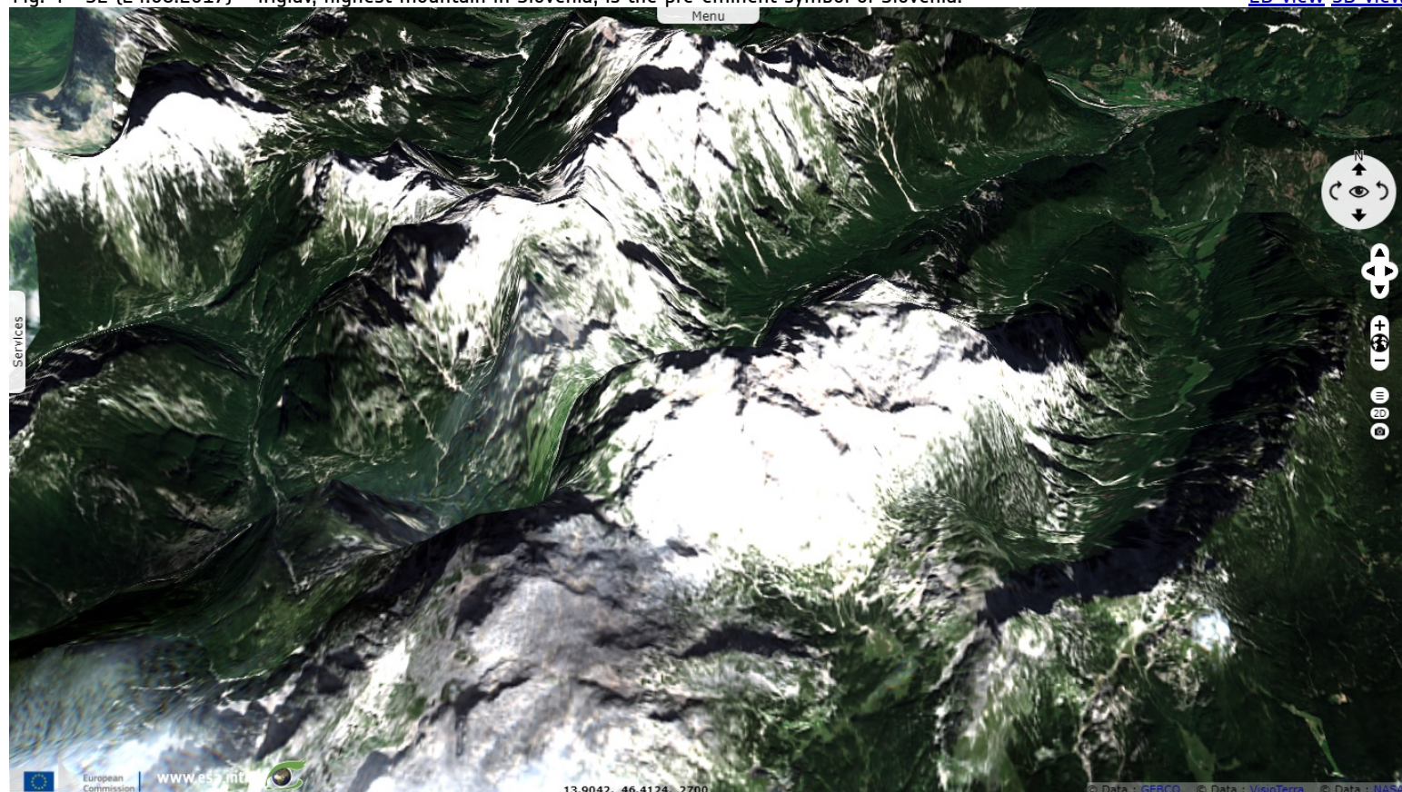
Fig. 4 - S2 (24.08.2017) - Triglav, highest mountain in Slovenia, is the pre-eminent symbol of Slovenia.
