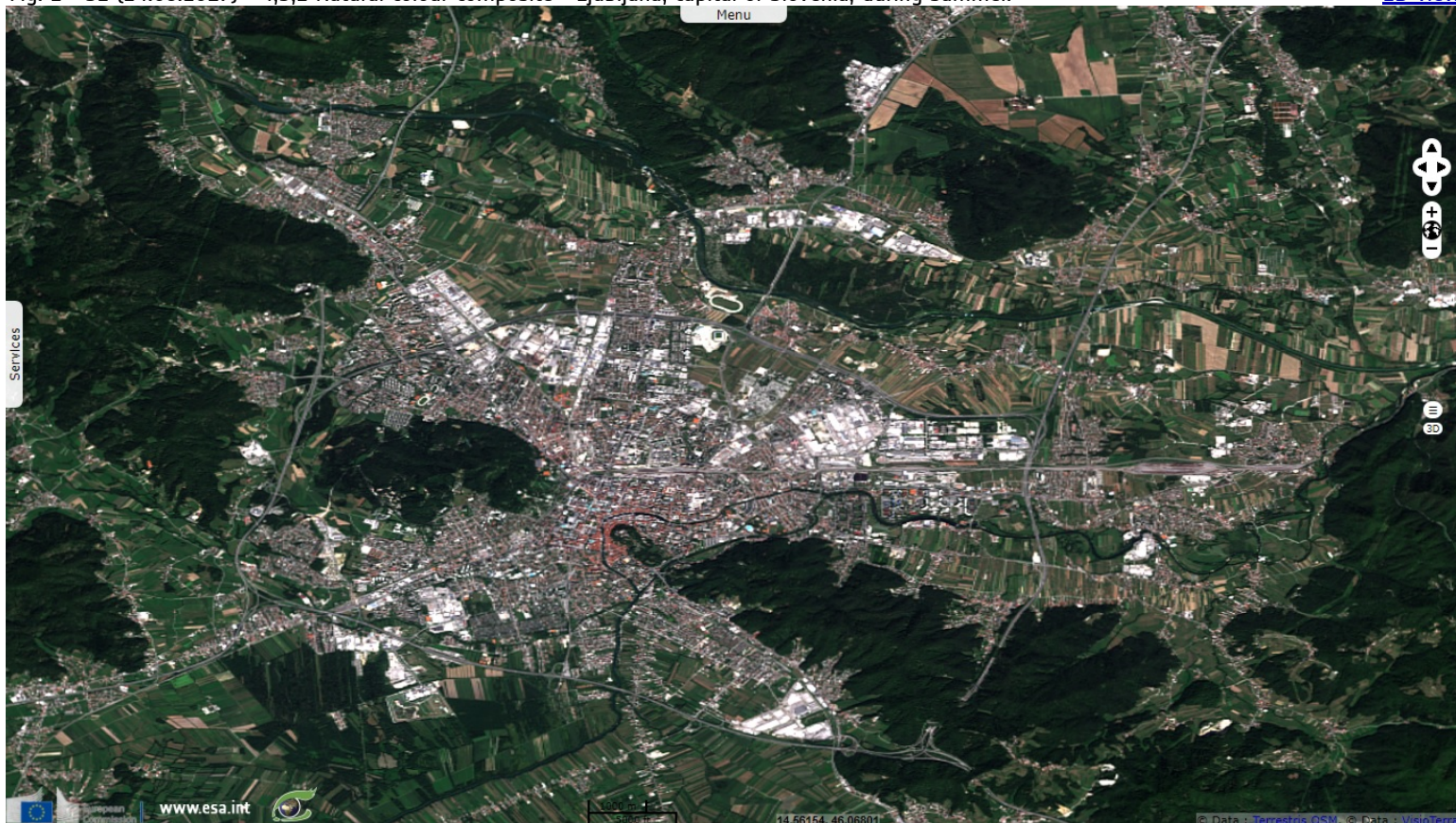
Fig. 2 - S2 (24.08.2017) - 4,3,2 Natural colour composite - Ljubljana, capital of Slovenia, during summer.
