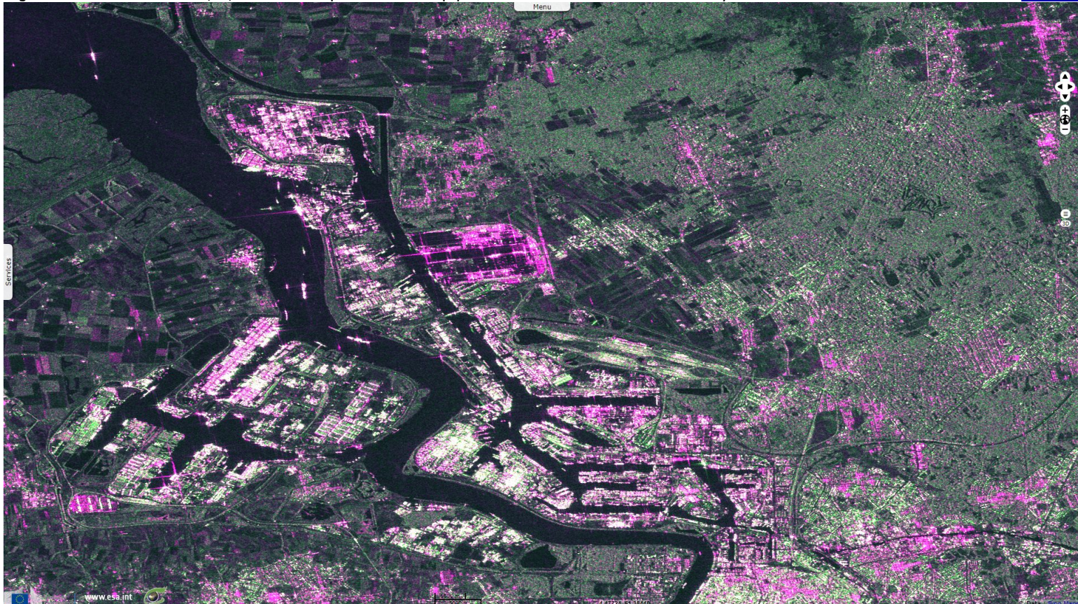
Fig. 2 - S1 (27.05.2017) - vv,vh,vv colour composite - Antwerp port is located downstream of the city centre.
