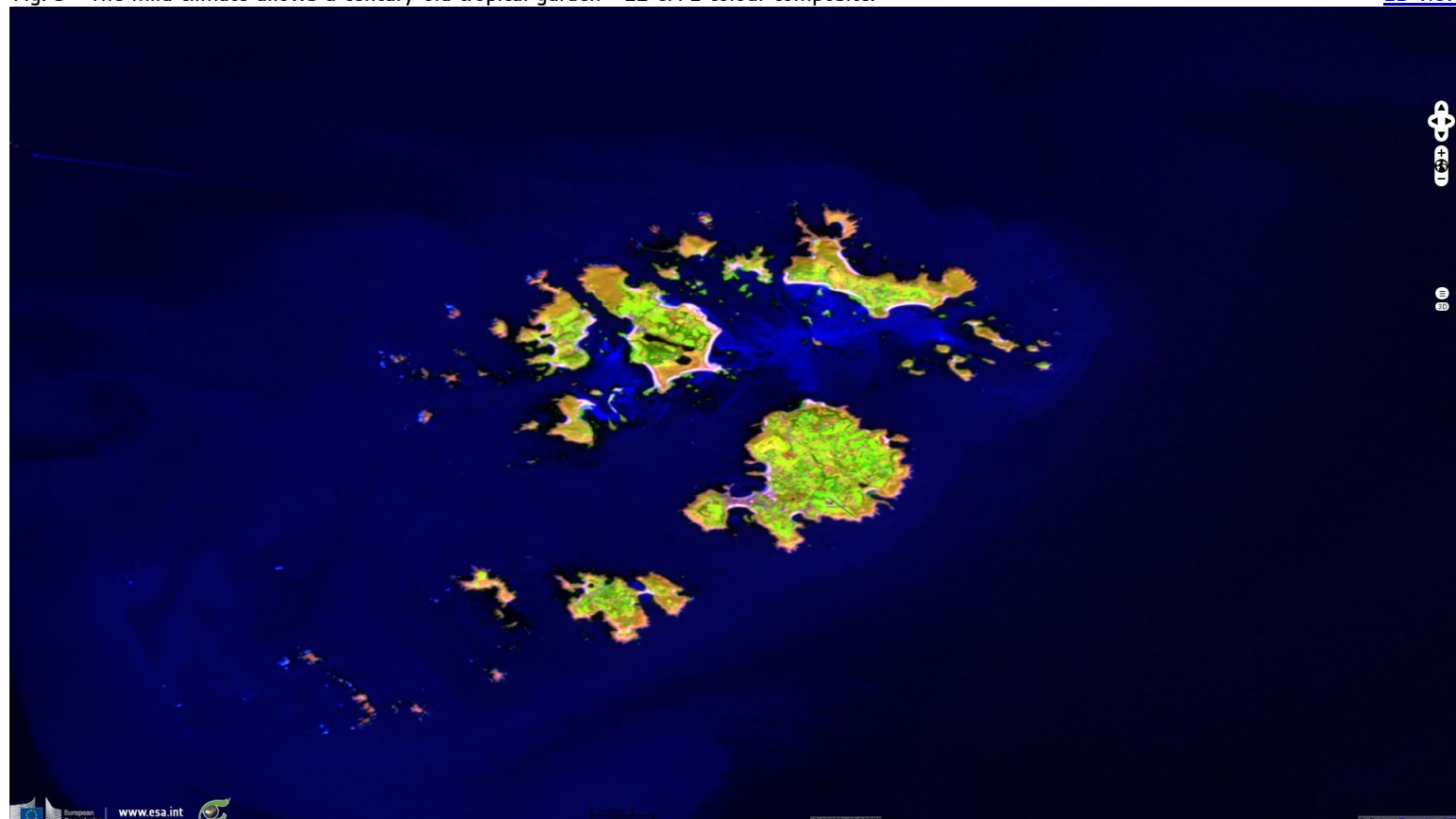
Fig. 4 - 2000 people live on this hundred of inlets, most from tourism - VV-VH-NDI(VH,VV) colour composite.
