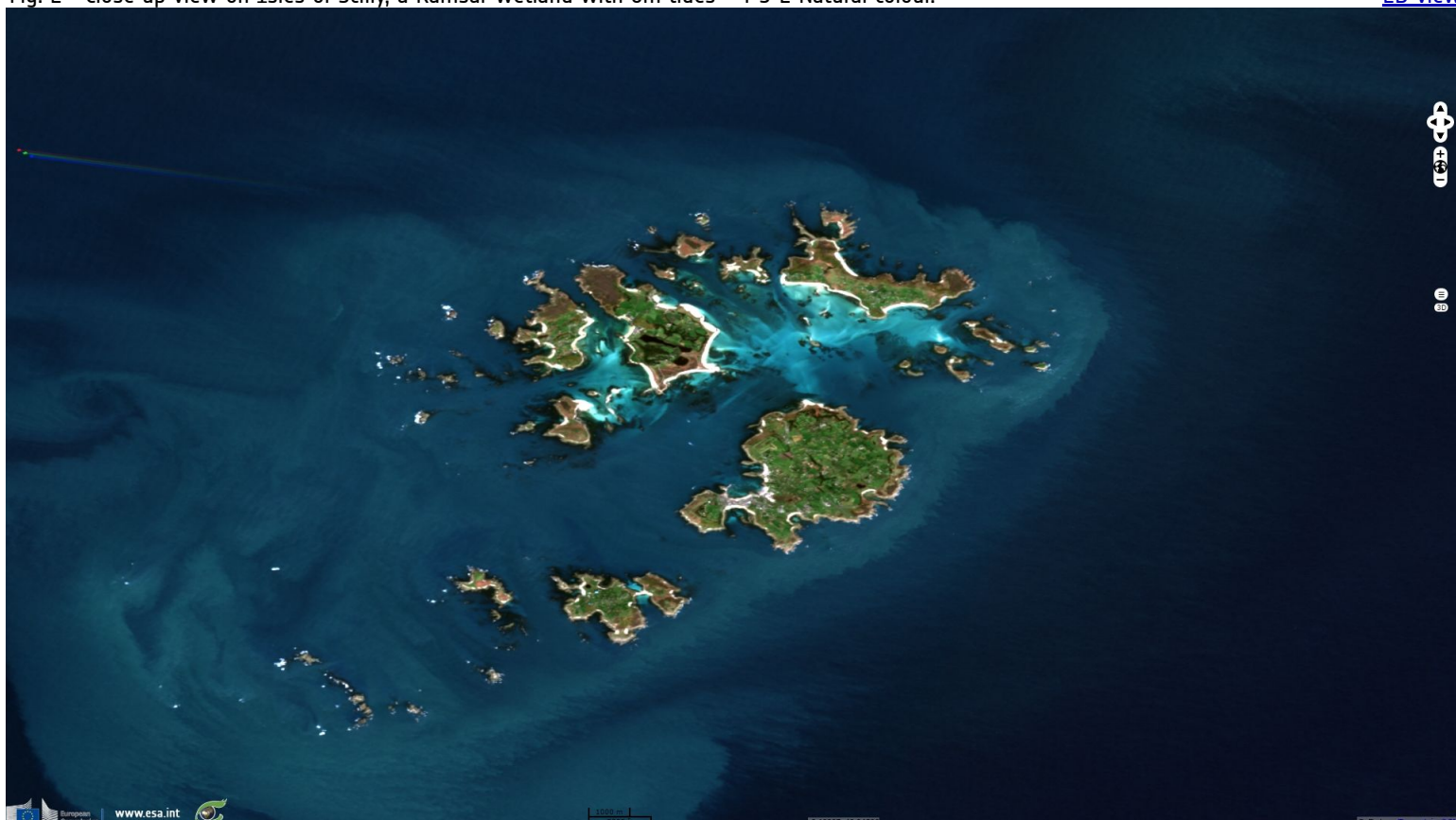
Fig. 2 - Close up view on Isles of Scilly, a Ramsar wetland with 6m tides - 4-3-2 Natural colour.
