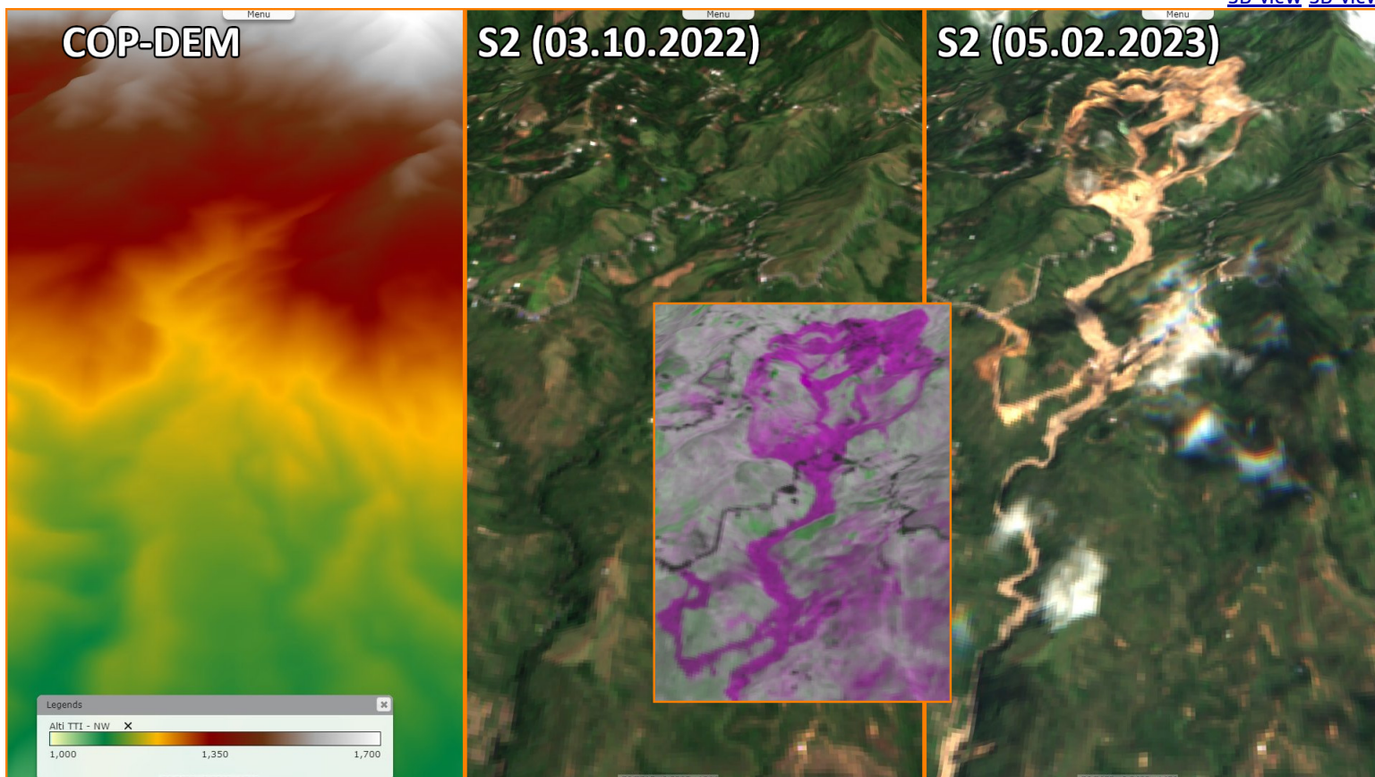
Fig. 1 - COP-DEM / S2 (03.10.2022 / 05.02.2023) - Since 09.01.2023, a 900 m x 850 m landslide has hit 3 villages in Rosas, Cauca.
