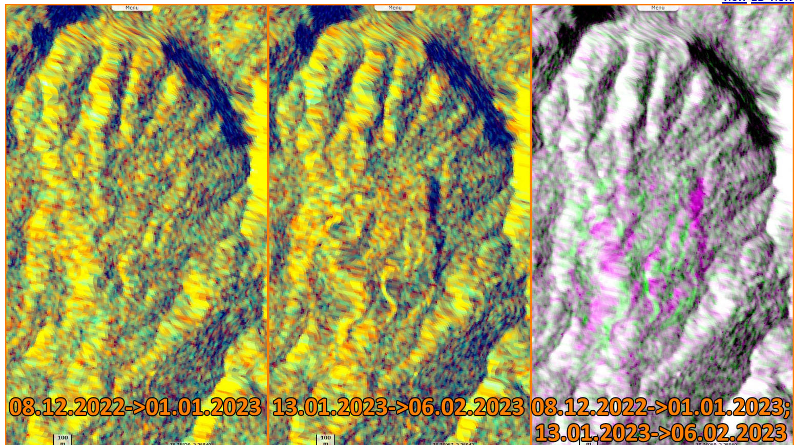
Fig. 2 - S1 (08.12.2022->01.01.2023; 13.01.2023->06.02.2023) - 64 homes have been destroyed, rendering over 700 people homeless. 2D view 2D view view 2D view
