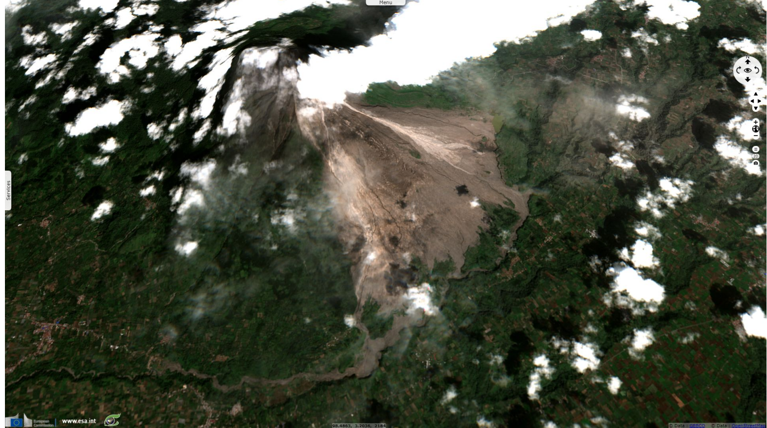
Fig. 4 - S2 (15.01.2018) - 12,11,2 colour composite - Lava flows from the erupting continuing in Jan. 2018. 3D view
