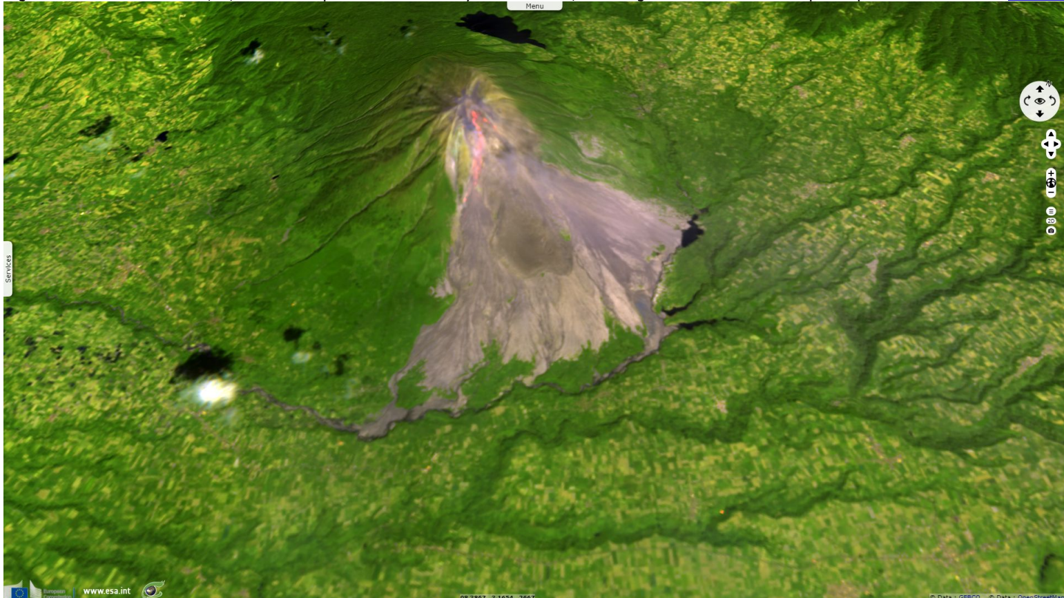
Fig. 2 - S2 (19.10.2017) - 12,11,2 colour composite - As shown by this lava flow, Sinabung underwent several eruptive episodes in 2017. 3D view
