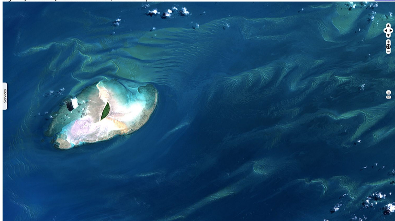
Fig. 4 - (13.04.2017) - Underwater dunes, southern Papua New Guinea.
