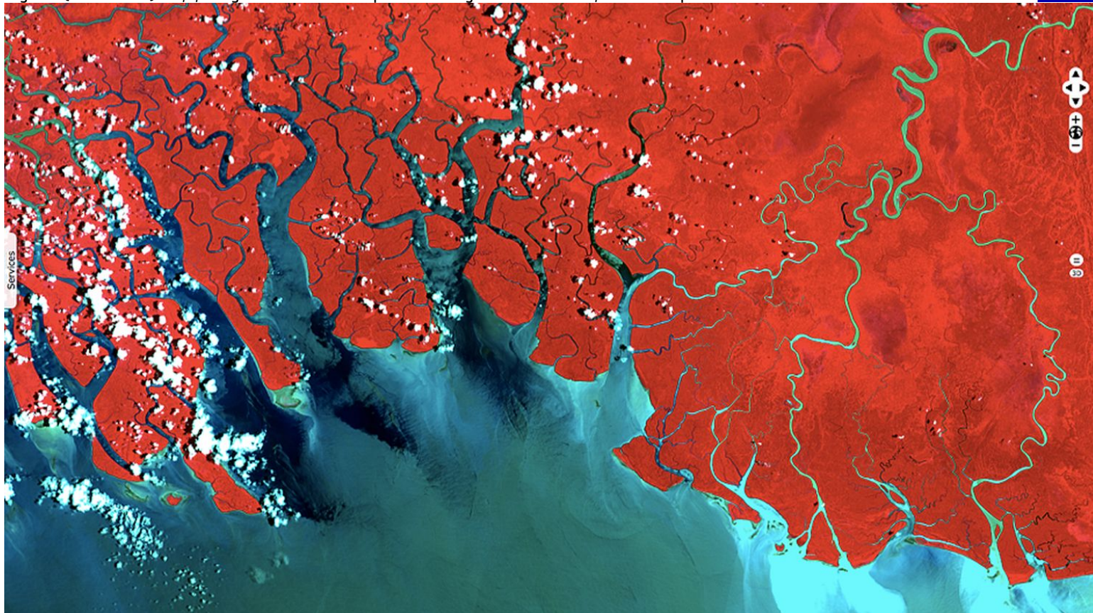
Fig. 2 - (12.02.2017) - 8,4,3 Vegetation colour composite - Mangroves near Kikori, eastern Papua New Guinea.
