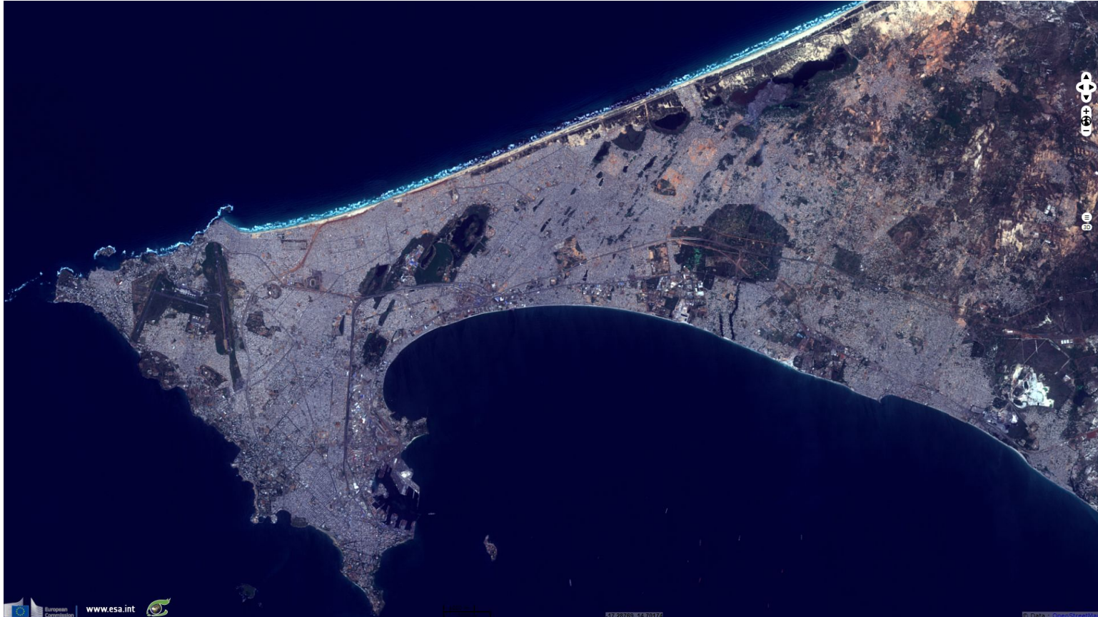
Fig. 1 - S2 (10.10.2017) - 4,3,2 natural colour - Founded in 1850s, Dakar now hosts 25% of Senegal population, 50% including its suburb. 2D view
