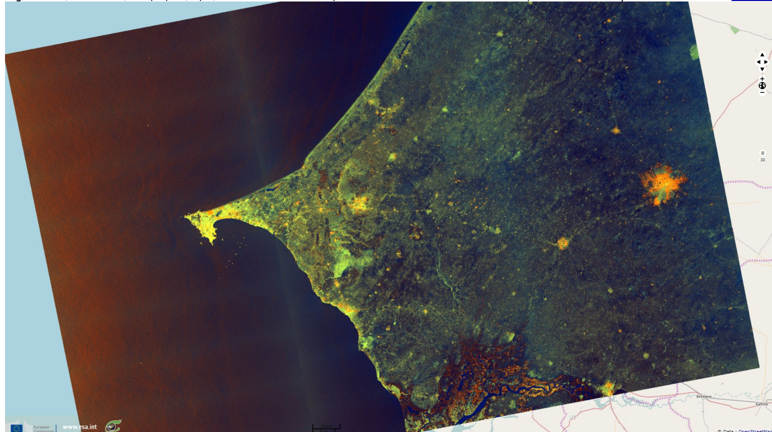
Fig. 4 - S1 (31.01.2017) - vv,vh,ndi(vh,vv) - Pointe des Almadies, westernmost land of mainland Africa, is home to an important oceanic front.
