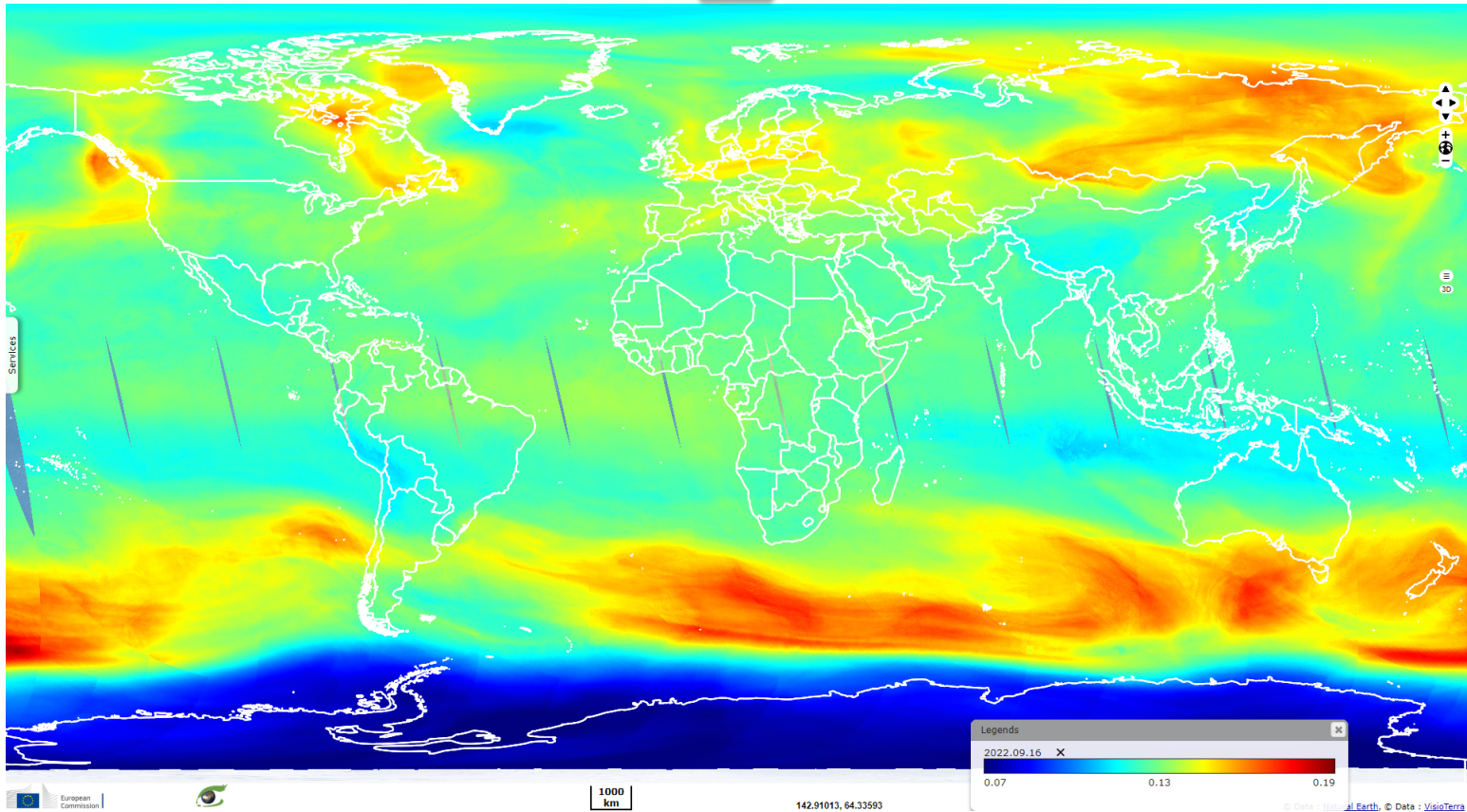
Fig. 1 - S5P TROPOMI (16.09.202) - Total ozone column - 16 September is the UN International Day for the Preservation of the Ozone Layer. 2D view
