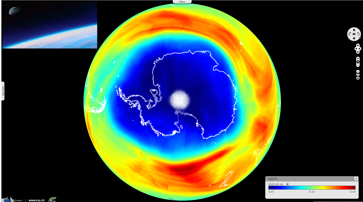
Fig. 2 - S5P TROPOMI (16.09.202) - The ozone hole above the Antarctic has become a global symbol of the environmental threat. 3D view
