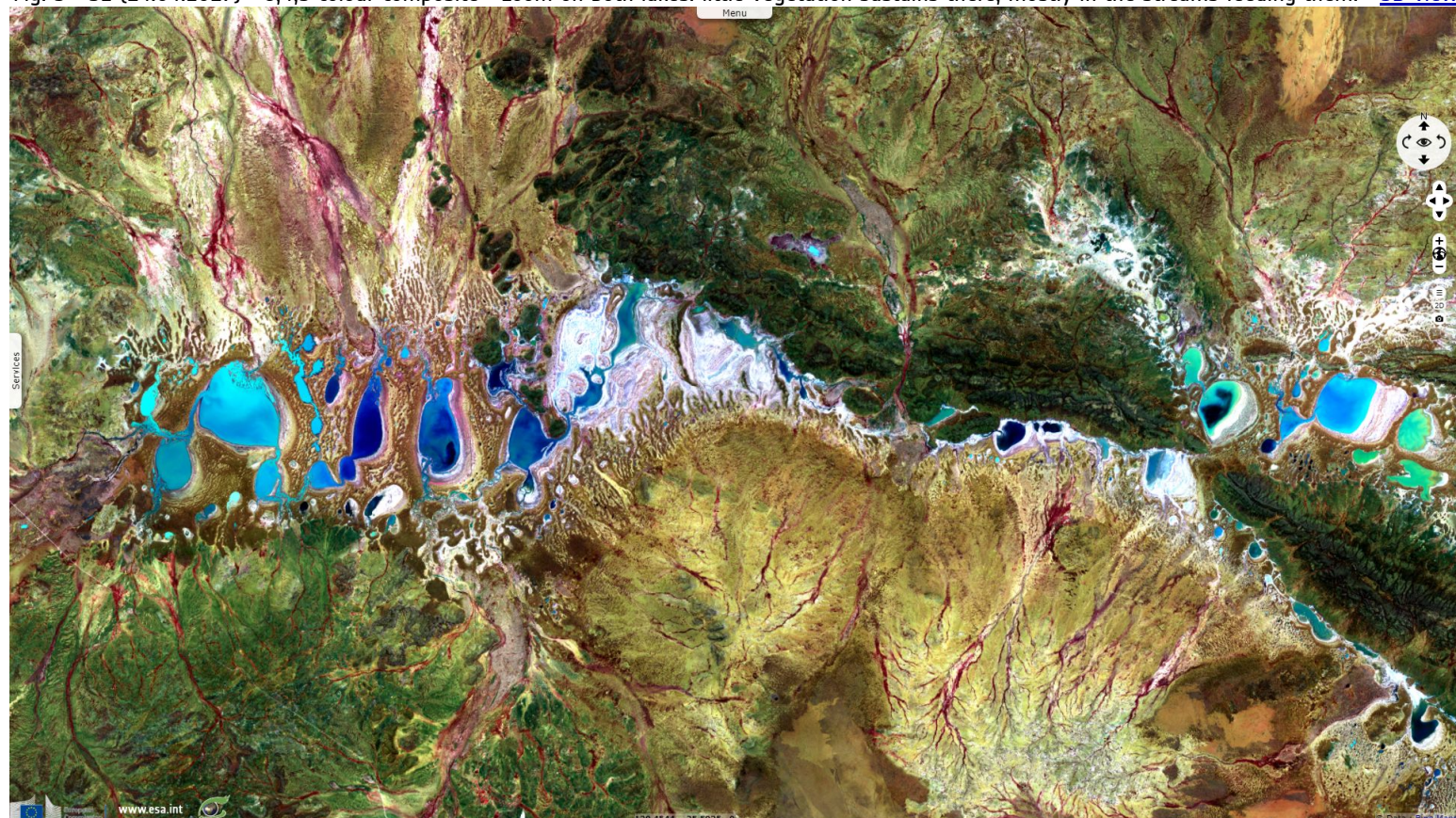
Fig. 4 - S1 (10.06.2018) - vv,vh,ndi(vh,vv) colour composite - The ponds of each lake are only fully connected when the water level is high. 3D view
