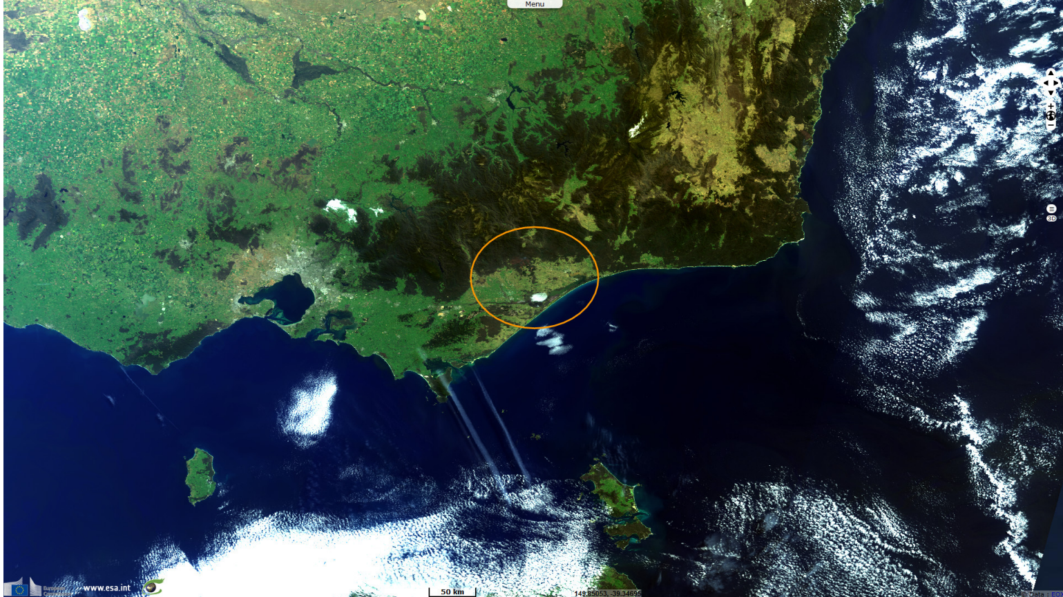
Fig. 2 - S3 OLCI (30.09.2023 and 01.10.2023) - The bushfire started on September 30 and threatened the rest of the forest, crops and towns. 2D view
