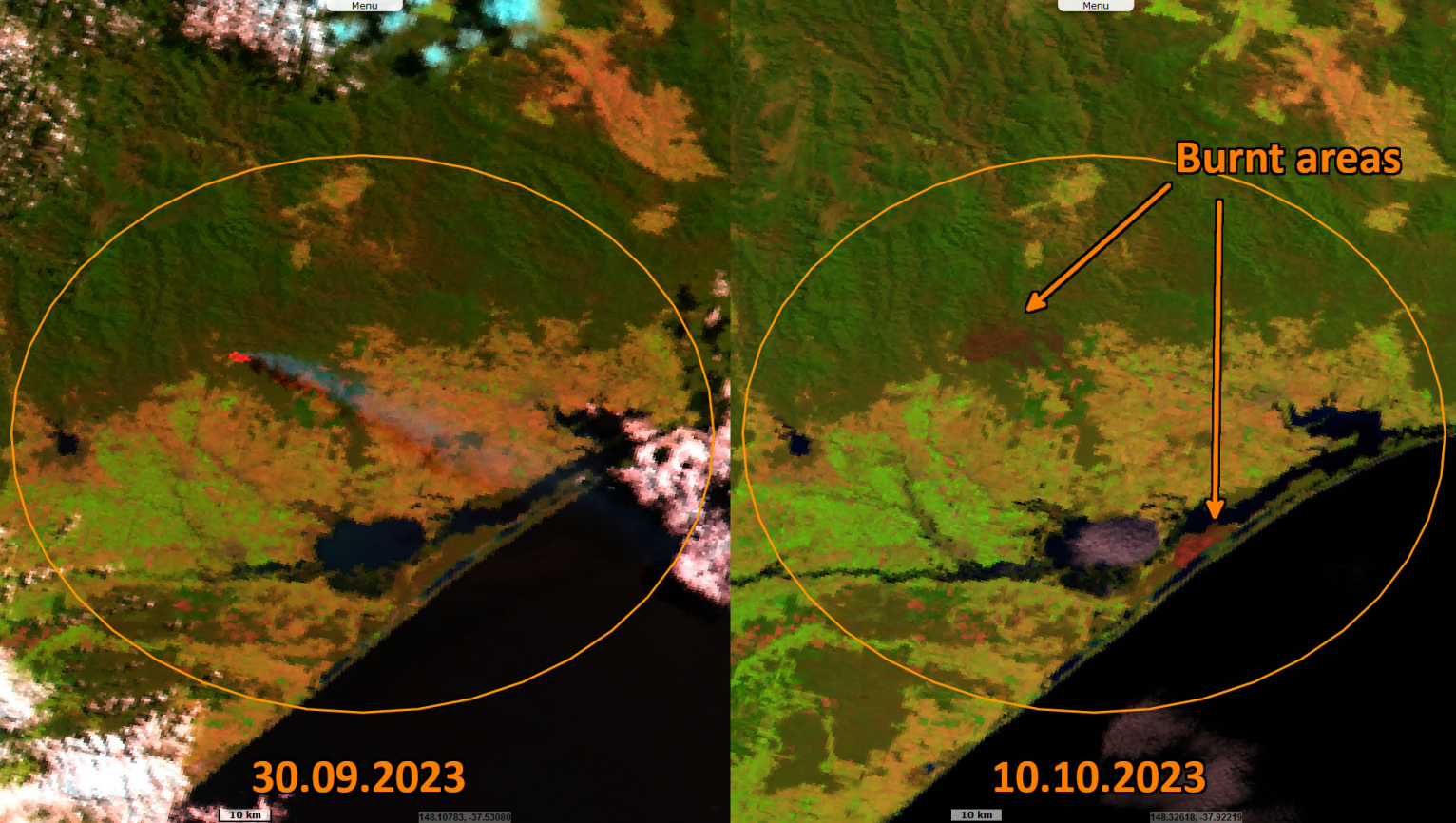
Fig. 5 - S3 SLSTR (30.09.2023 and 10.10.2023) - Significant rainfall helped extinguish the fires before they spread to the rest of the forest. 2D view
