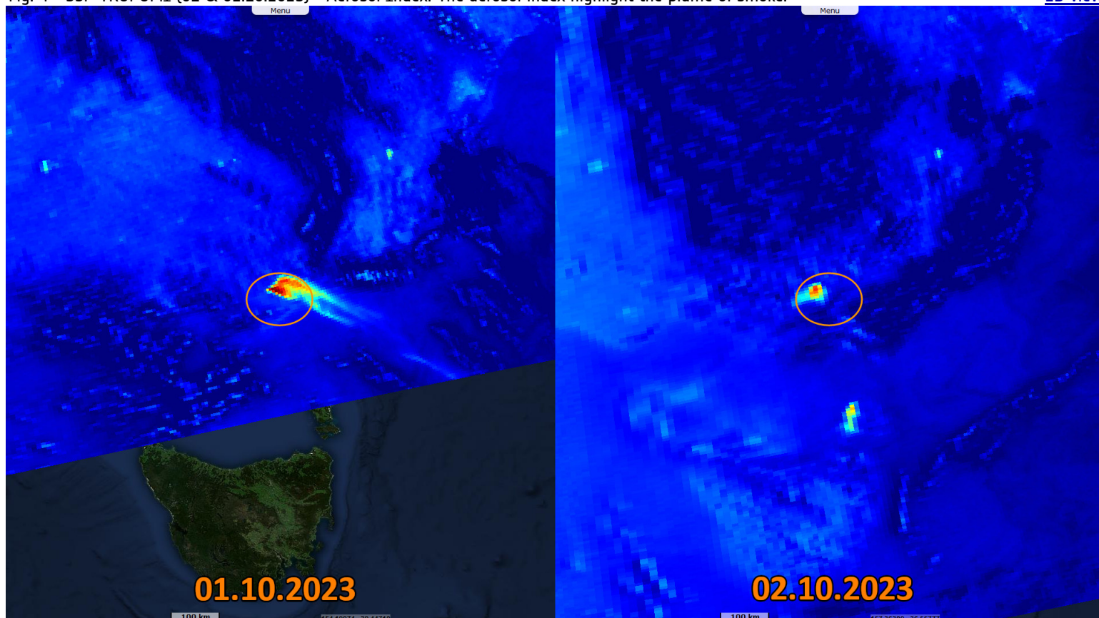
Fig. 4 - S5P TROPOMI (01 & 02.10.2023) - Aerosol Index. The aerosol index highlight the plume of smoke.
