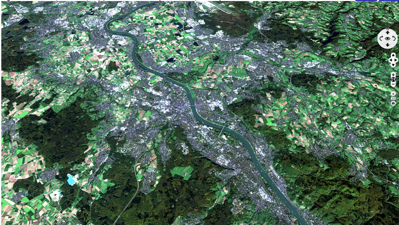
Fig. 2 - Sentinel 2A (15.10.2017) - 4,3,2 Natural colour composite - Bonn, Germany.
