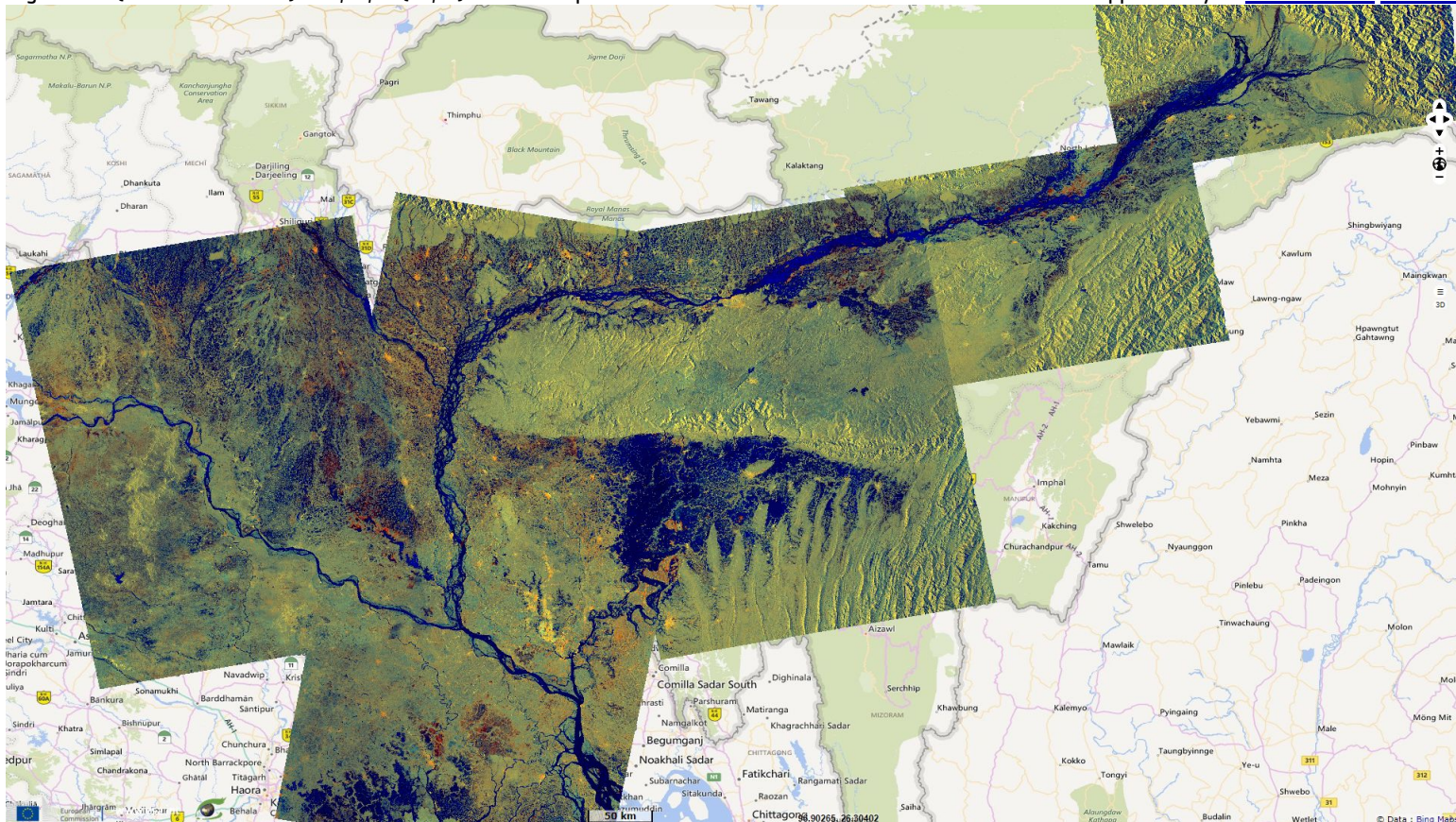
Fig. 2 - S1 (09 to 16.07.2019) - vv,vh,ndi(vh,vv) colour composite - Same after the monsoon rain overflowed the upper valley.
