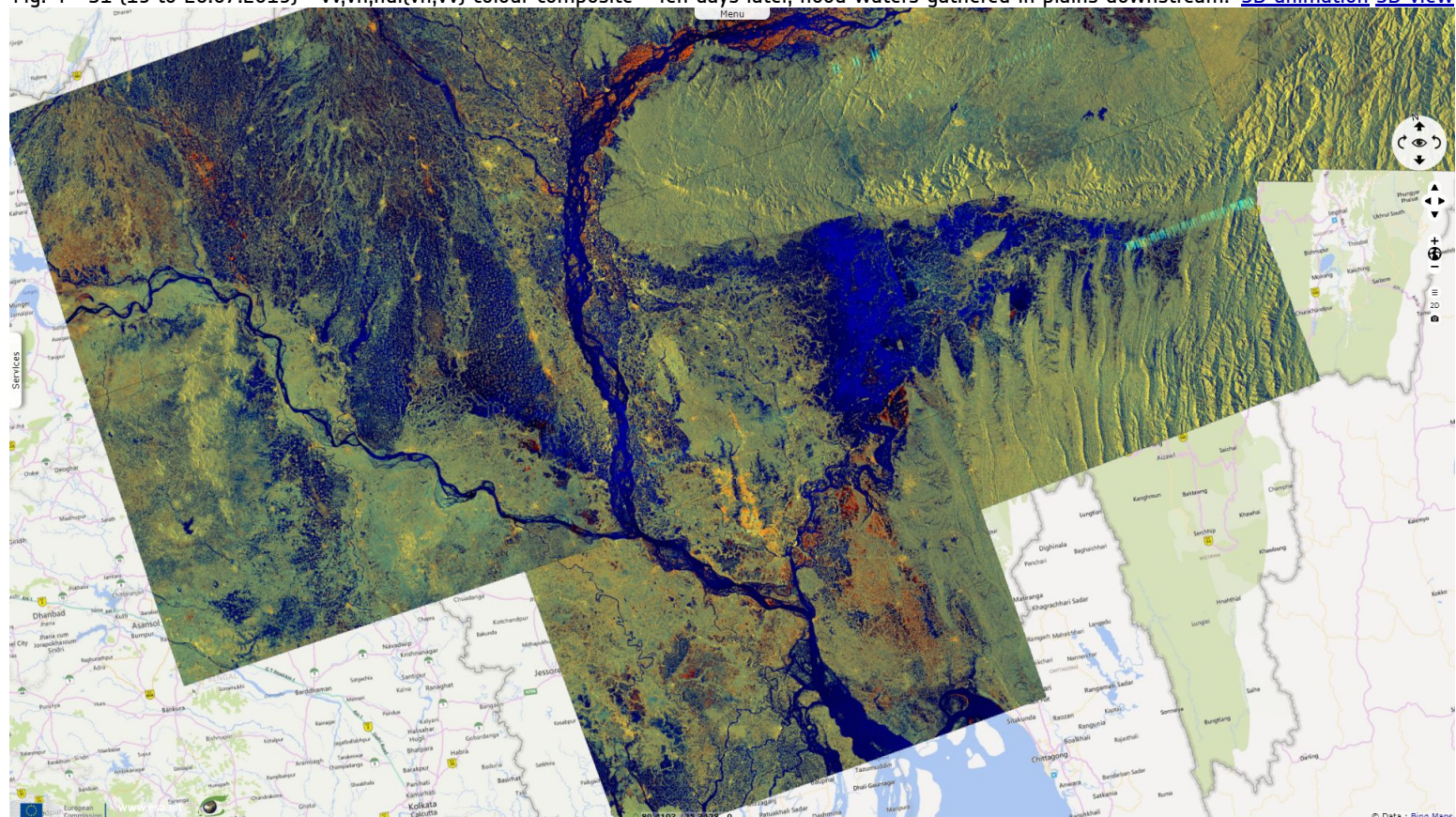
Fig. 4 - S1 (19 to 26.07.2019) - vv,vh,ndi(vh,vv) colour composite - Ten days later, flood waters gathered in plains downstream.
