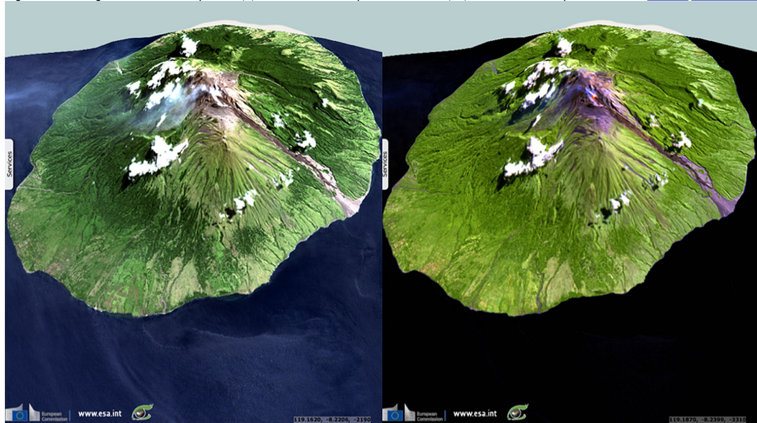
Fig. 4 - Pulau Sangeand volcano in eruption - 4,3,2 Natural colour composite (left) vs. 12,11,4 Urban colour composite.
