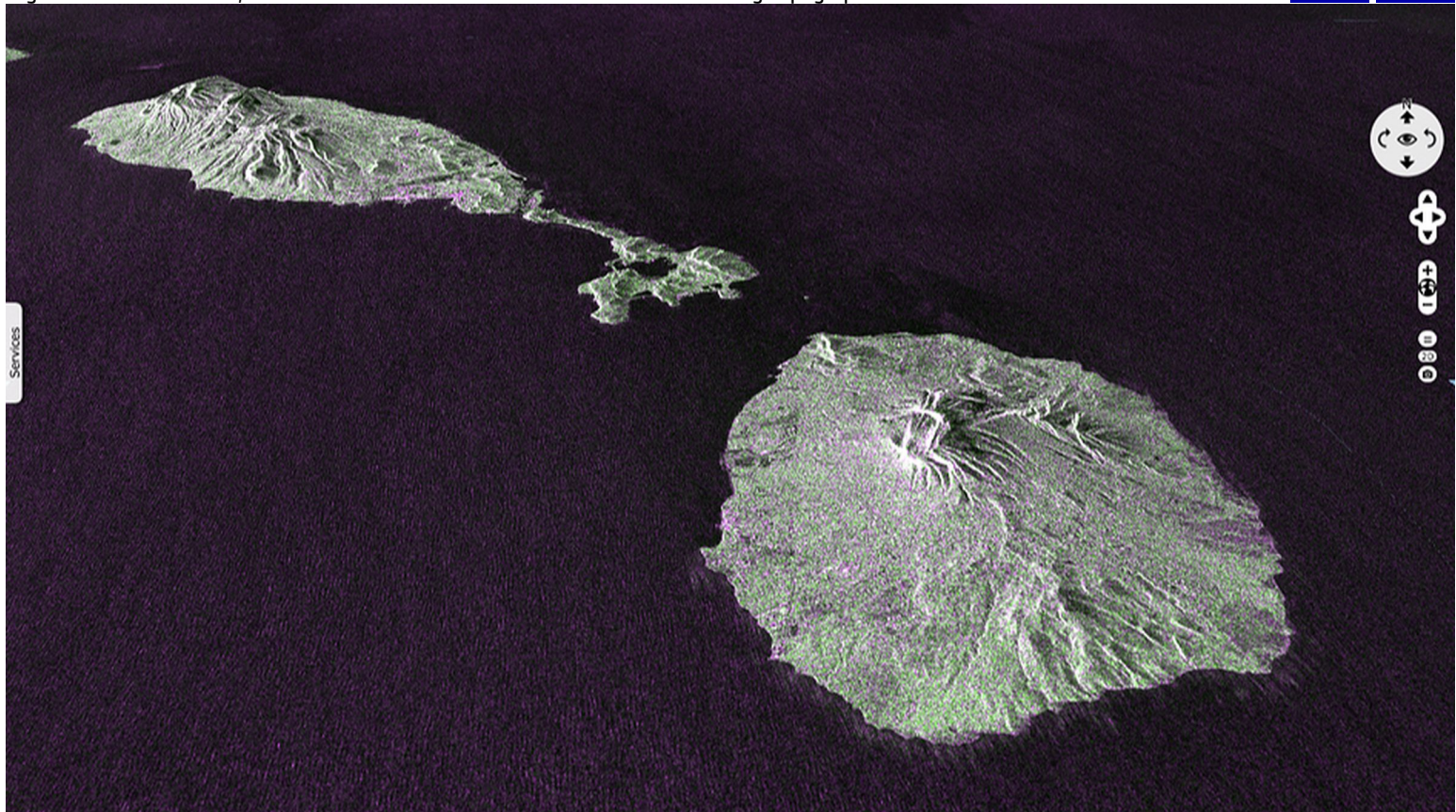
Fig. 2 - Sentinel 1A - vv, vh raw - 06.09.2017 - Volcano craters and interesting topographic structures.
