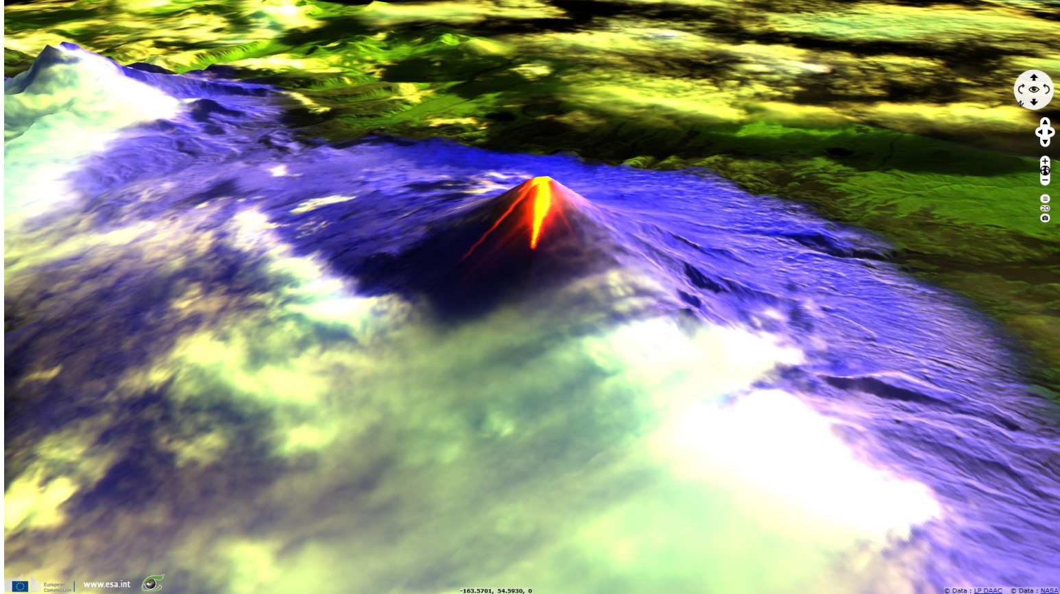
Fig. 2 - S2 (29.10.2019) - 12,11,4 colour composition - The mount Shishaldin after the eruption.
