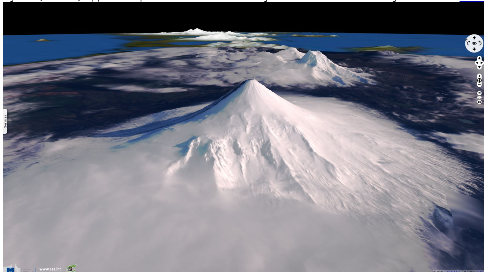
Fig. 4 - S1 (30.10.2019) - vv,vh,ndi(vh,vv) - The mount Shishaldin reaches the altitude of 2857m.
