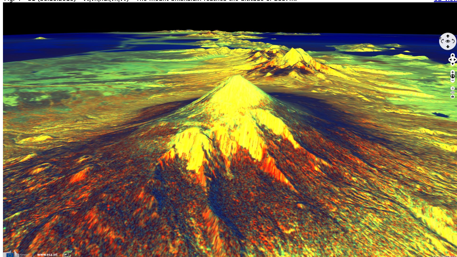
Fig. 4 - S1 (30.10.2019) - vv,vh,ndi(vh,vv) - The mount Shishaldin reaches the altitude of 2857m.
