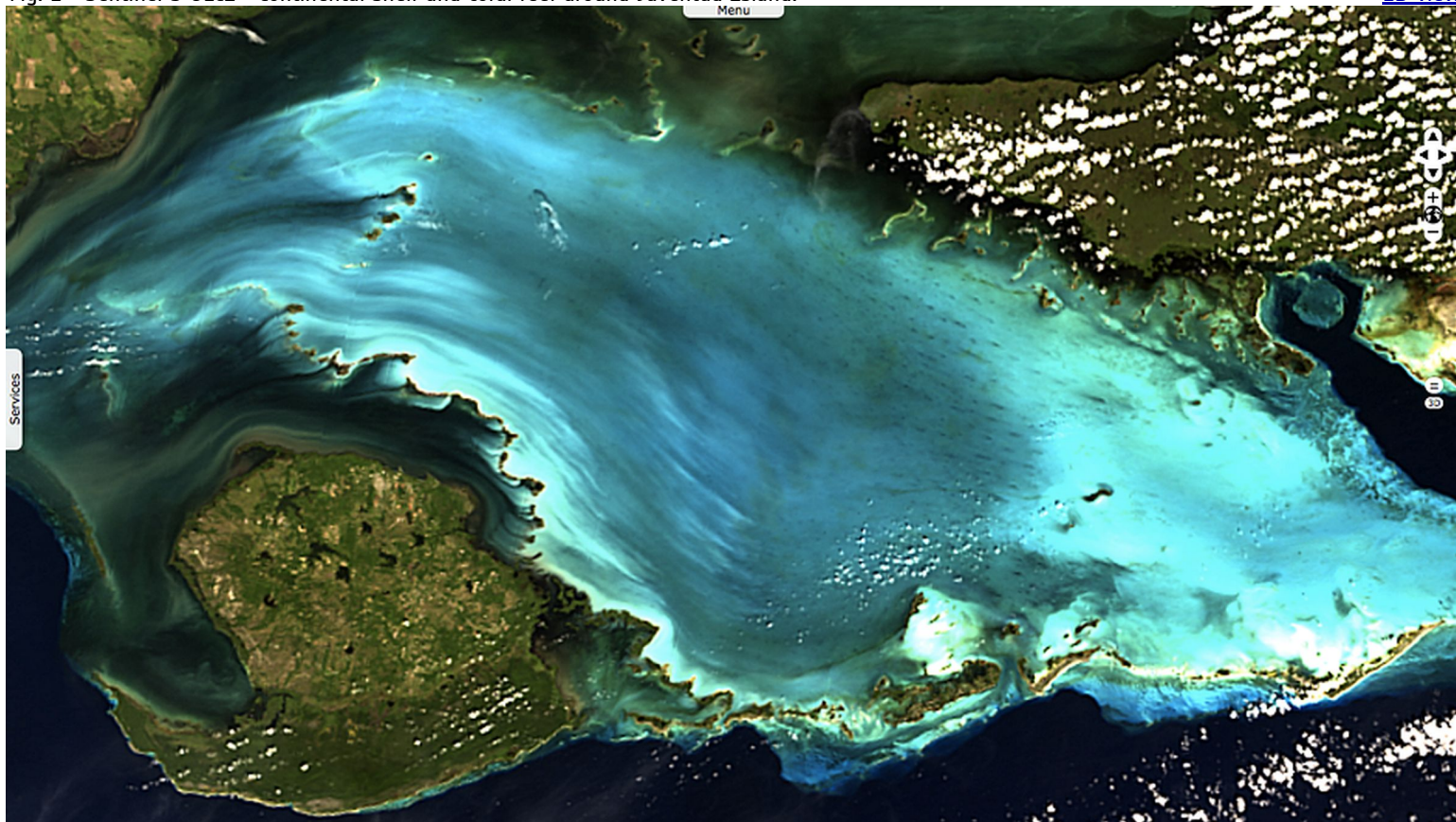
Fig. 2 - Sentinel 3 OLCI - Continental shelf and coral reef around Juventud Island.
