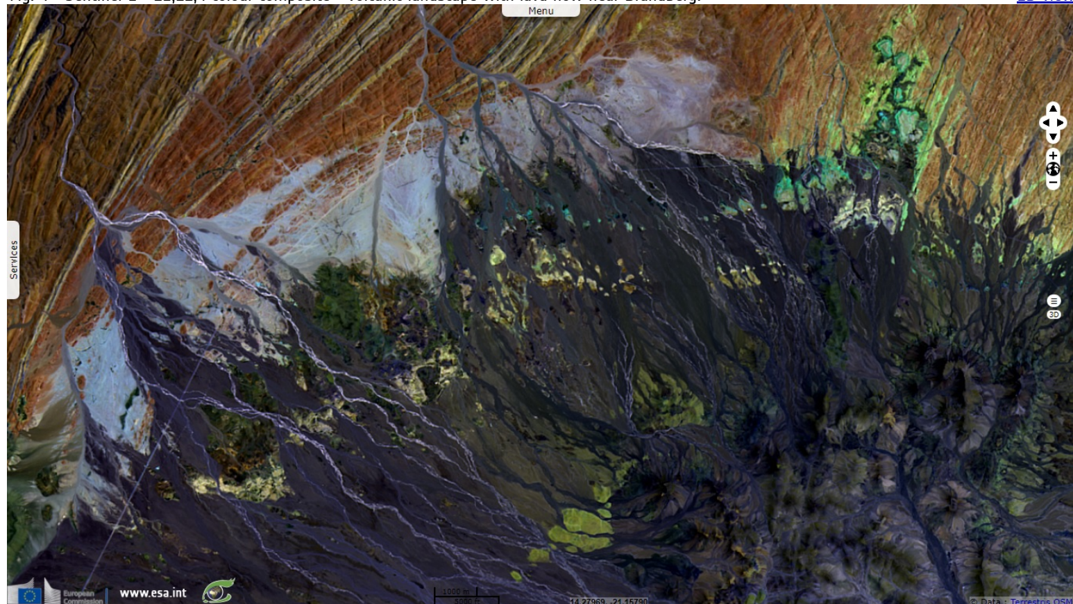
Fig. 4 - Sentinel-2 - 12,11,4 colour composite - Volcanic landscape with lava flow near Brandberg.
