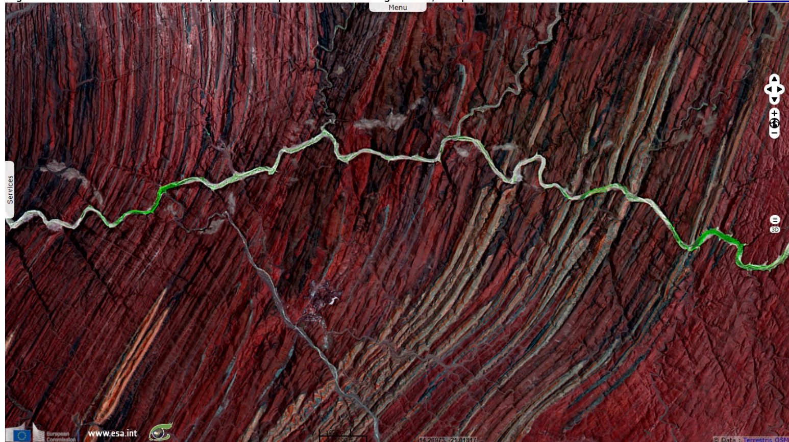
Fig. 4 - Sentinel-2 - 12,11,4 colour composite - Volcanic landscape with lava flow near Brandberg.
