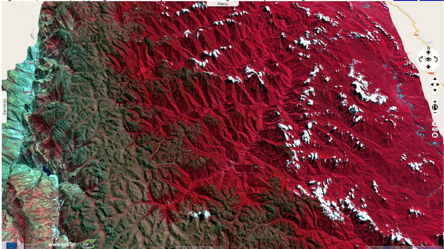
Fig. 2 - S2 (23.07.2017) - 8,4,3 Vegetation colour composite - Nuances in vegetation composition along the Andean Cordillera.
