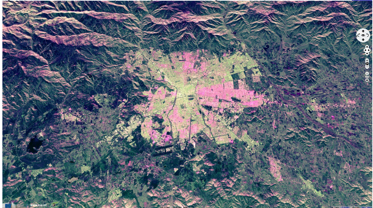
Fig. 4 - S2 (26.09.2019) - Finally, Spain offered to host the event; participants should define how they implement the Paris Agreement goals. 3D view
