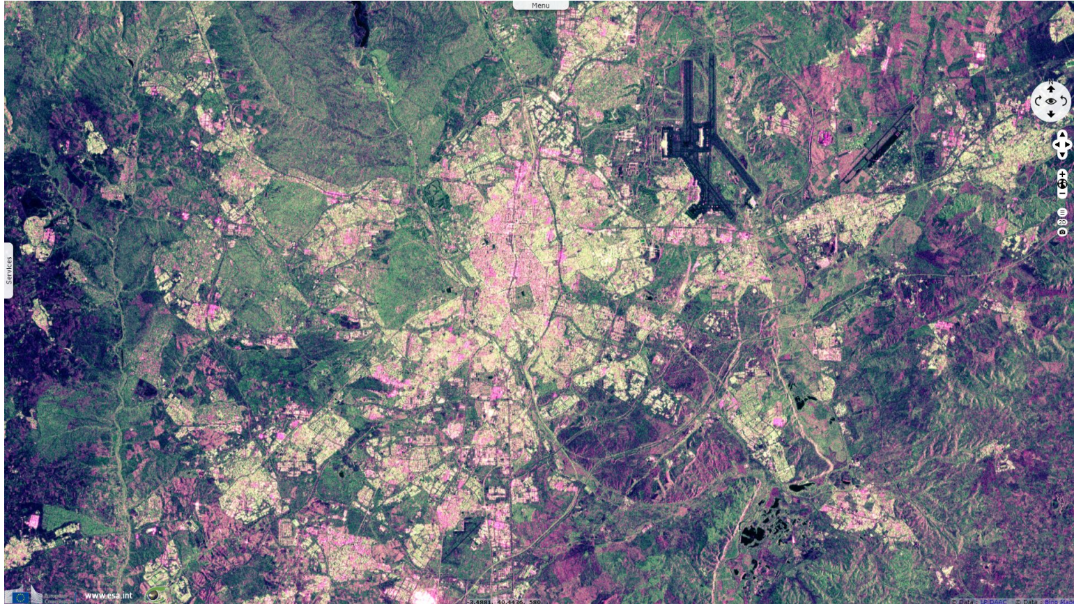
Fig. 1 - S1 (21.09.2019) - vv,vh,vv colour composite - Madrid hosts the 25th Conference Of the Parties held 2-13 December 2019.
