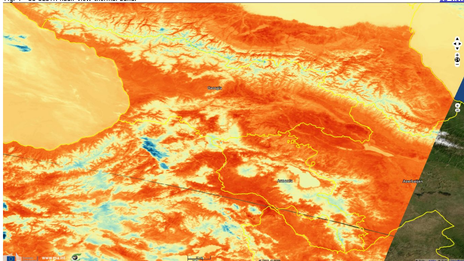
Fig. 4 - S3 SLSTR nadir view thermal band.
