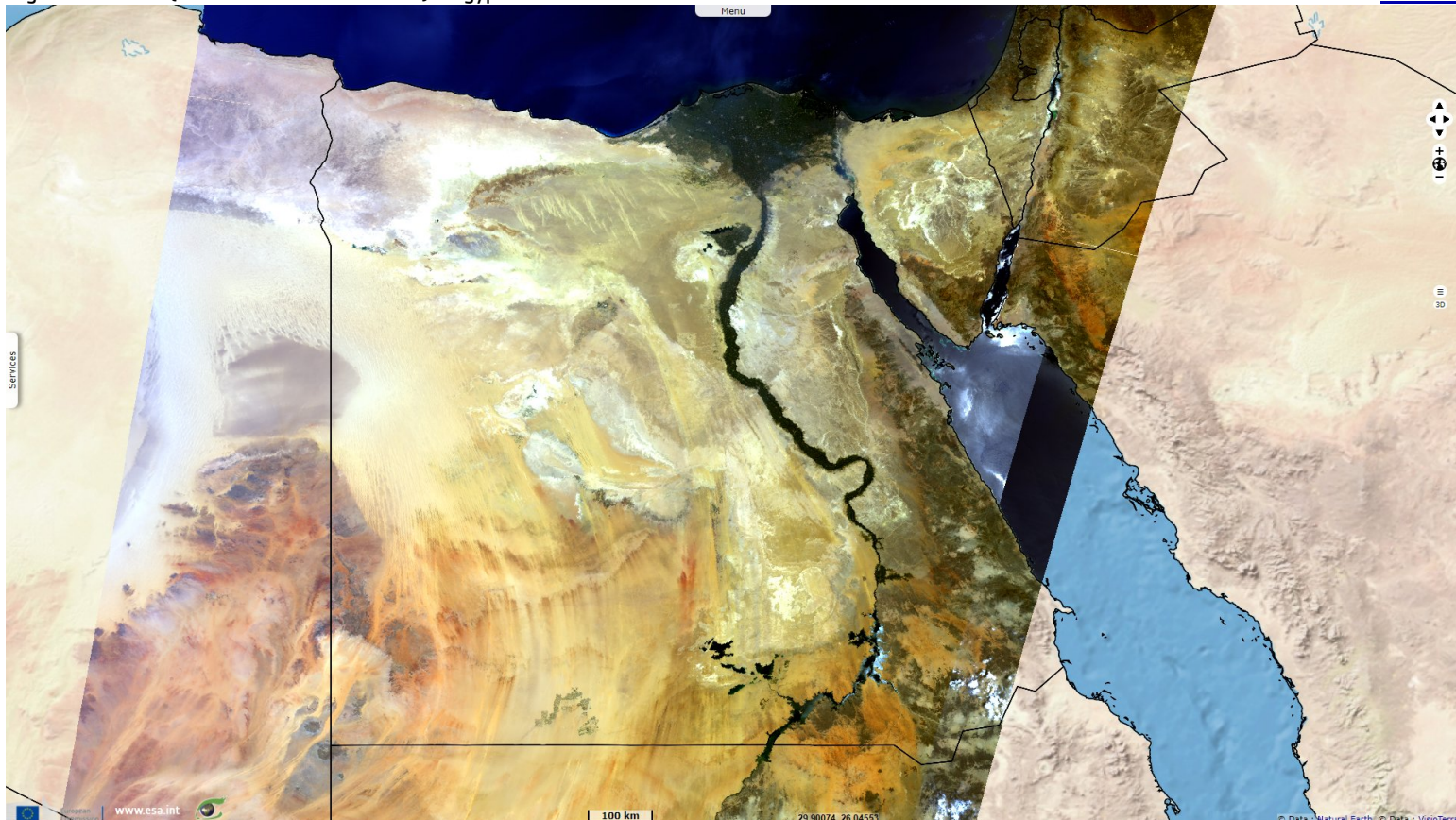
Fig. 2 - S3 OLCI (01.08.2021 & 01.09.2021) - Egypt reached the finals but failed to add an 8th AfCON title.
