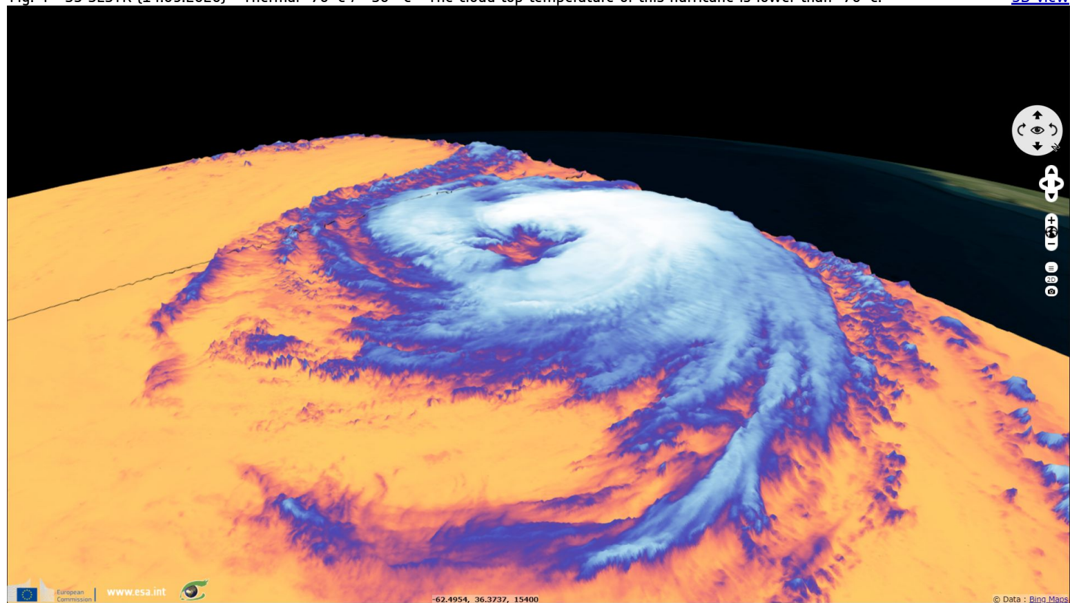
Fig. 4 - S3 SLSTR (14.09.2020) - Thermal -70°C / +30 °C - The cloud top temperature of this hurricane is lower than -70°C. 3D view
