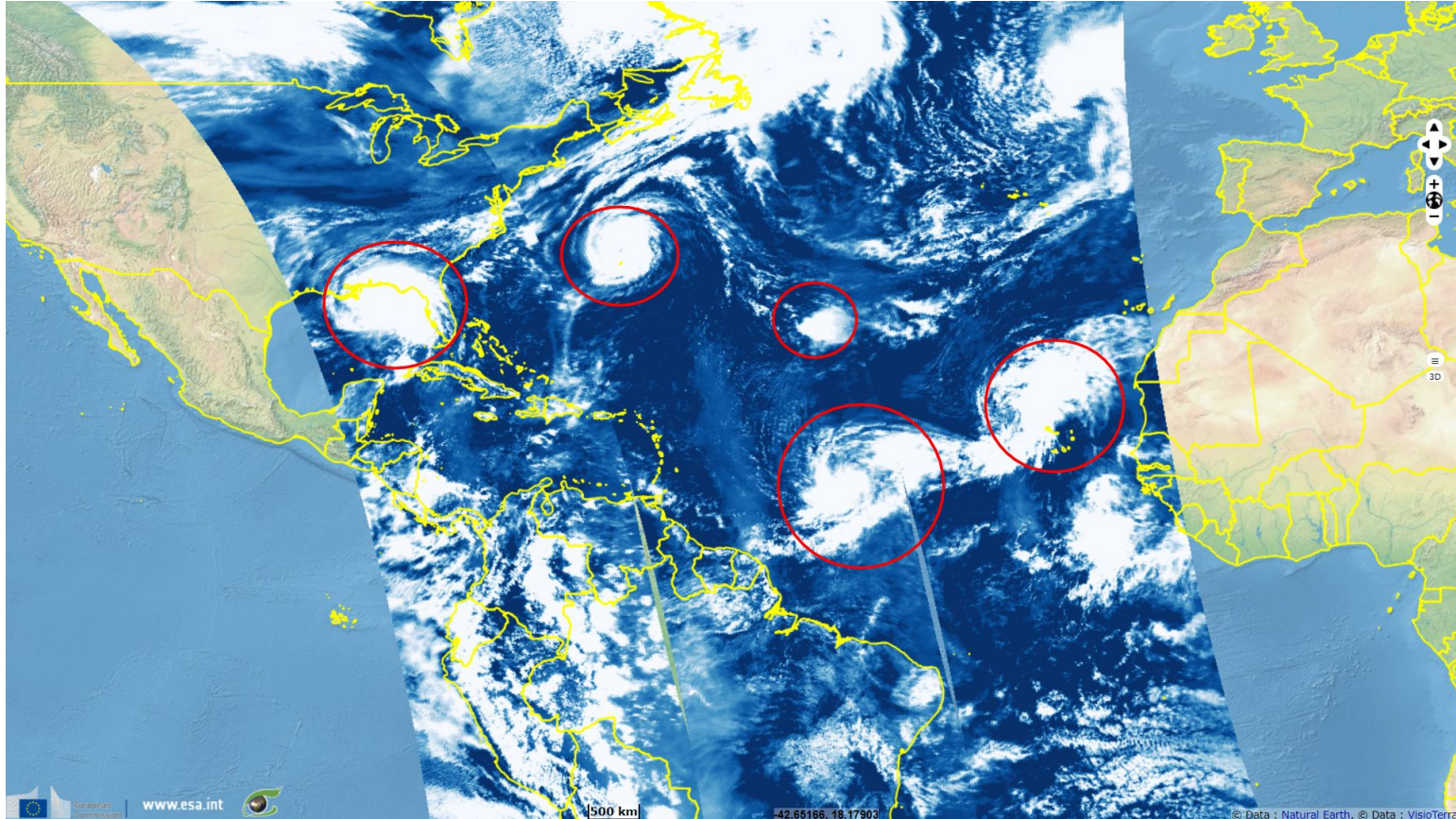
Fig. 2 - S3 OLCI (14.09.2020) - 10,6,3 colour composite - Global optical view through the reduced resolution of Sentinel-3 OLCI instrument. 3D view
