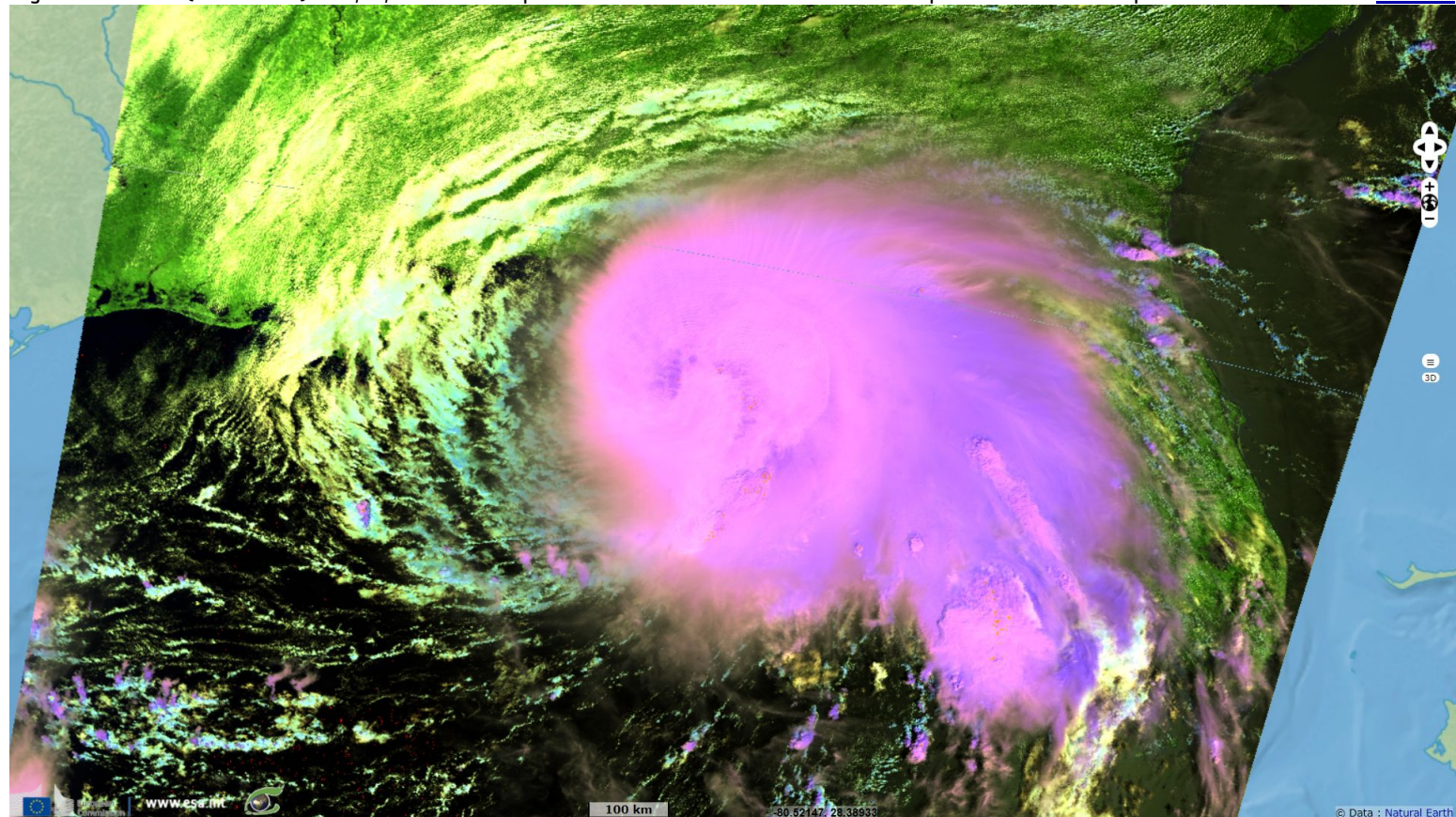
Fig. 4 - S3 SLSTR (14.09.2020) - Thermal -70°C / +30 °C - The cloud top temperature of this hurricane is lower than -70°C. 3D view
