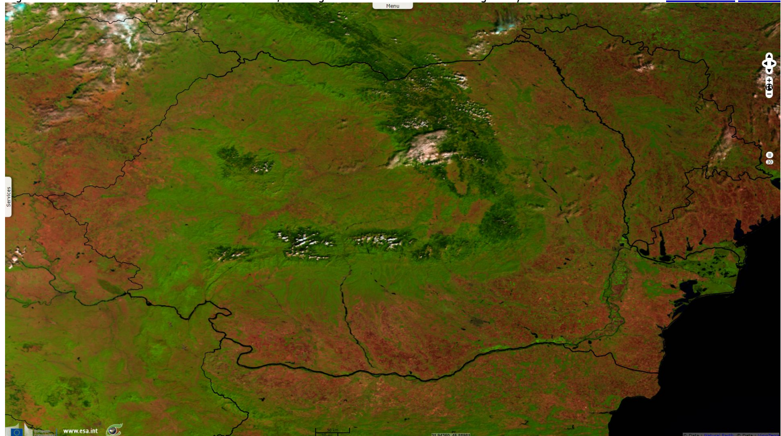
Fig. 4 - 27.08.2017 - The Carpathians cross Romania, drawing an inverted S extended in Bulgaria by the Balkans. 2D animation 2D view
