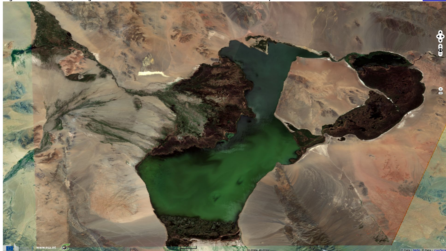
Fig. 4 - S2 (10 to 17.06.2017) - The shallow endorheic Uvs lake used to be a sea. It is the largest lake in Mongolia and a saline Ramser site.
