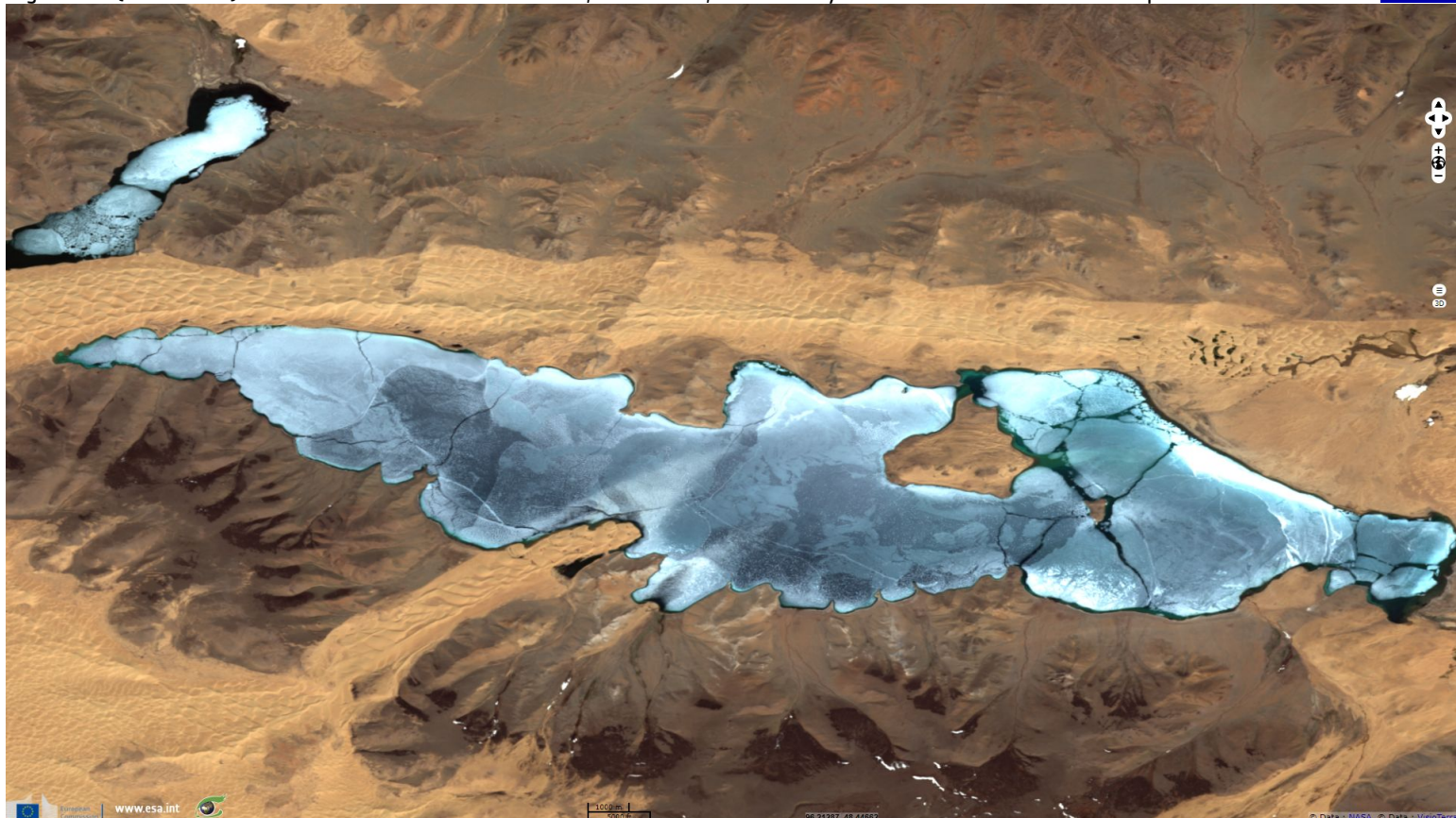
Fig. 2 - S2 (15.05.2017) - 4-3-2 - Natural colour - Khar Lake, here frozen, one of many endorheic lakes of the desertic plateau.
