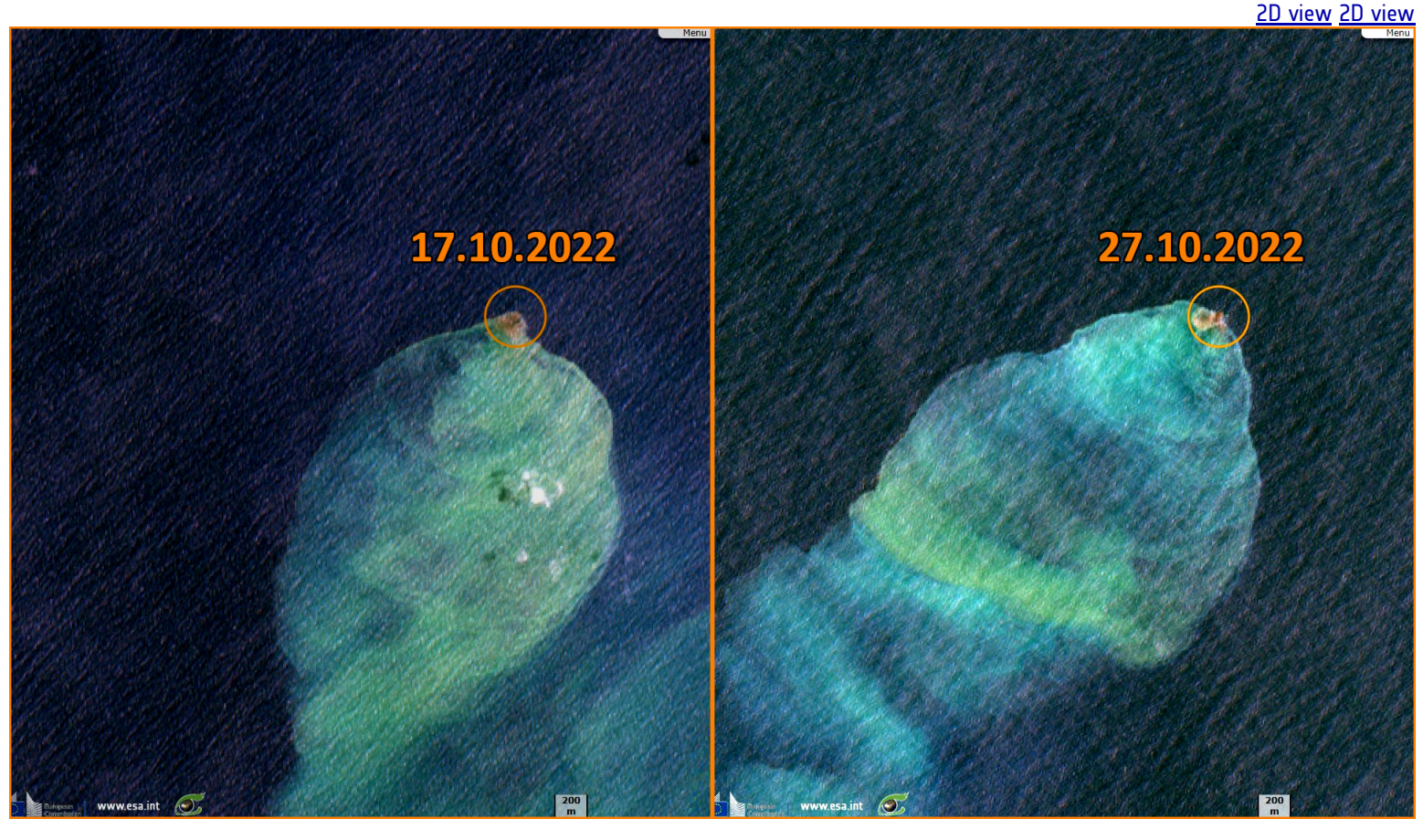
Fig. 3 - S2 (17.10.2022 / 27.10.2022) - Distinct yellow-green water in the vicinity of the submarine Kavachi volcano are indicative of the underwater eruptive episodes.
