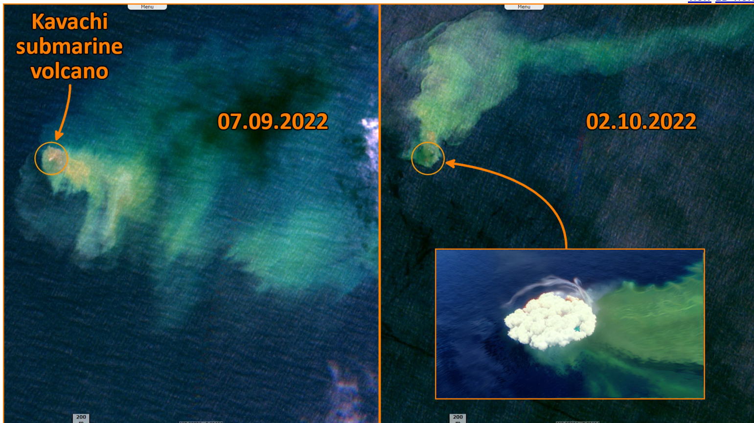
Fig. 2 - S2 (07.09.2022 / 02.10.2022) - Its volcanism is characterized by phreatomagmatic explosions ejecting steam, ash & incandescent bombs. 2D view 2D view
