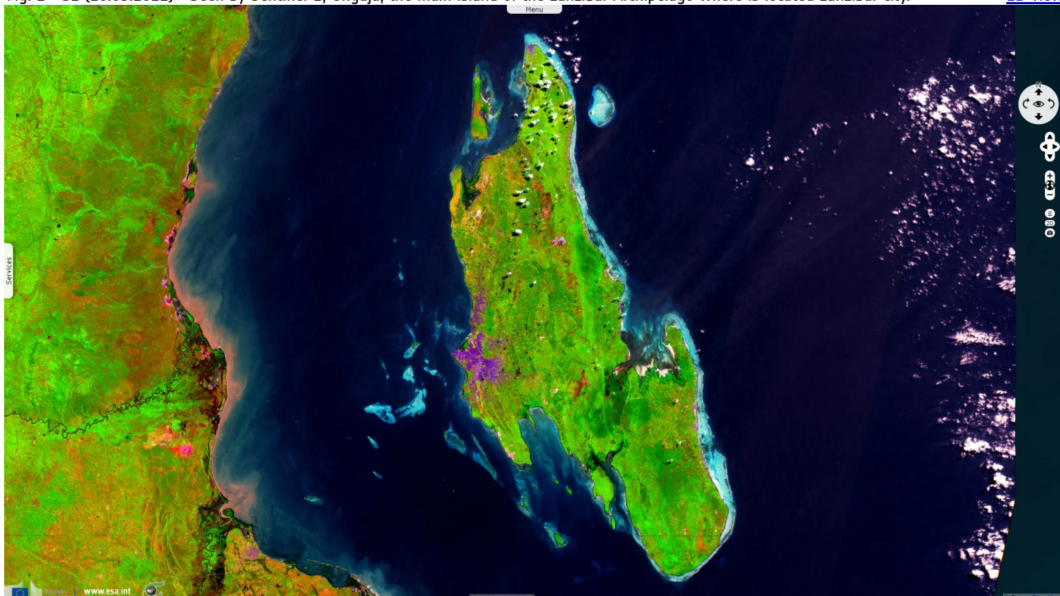
Fig. 2 - S2 (20.05.2021) - Seen by Sentinel-2, Unguja, the main island of the Zanzibar Archipelago where is located Zanzibar city.
