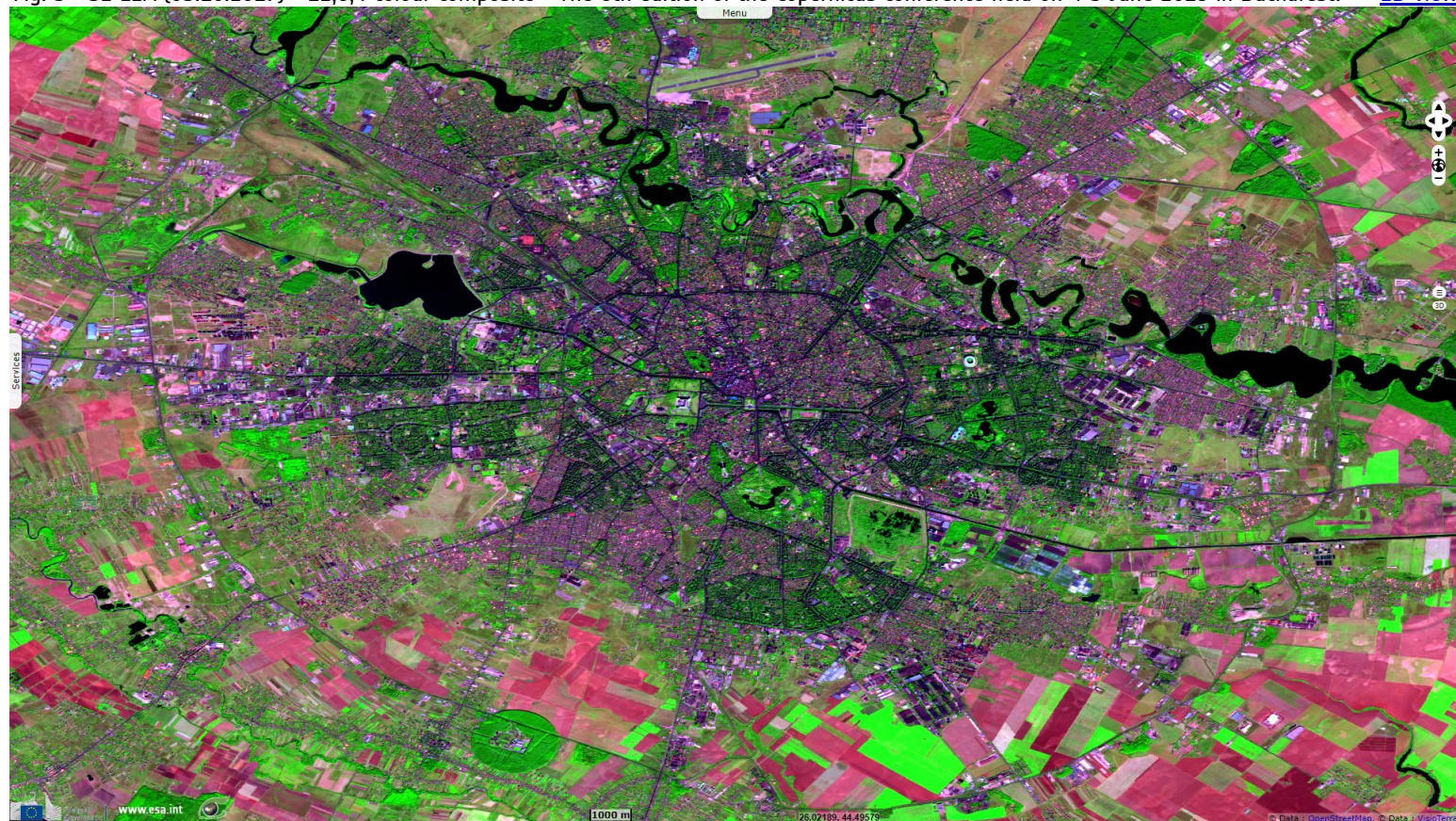
Fig. 4 - 4,3,2 natural colour - This year's edition is entitled "Space for a Secure Society and Sustainable Development". 2D view 3D view
