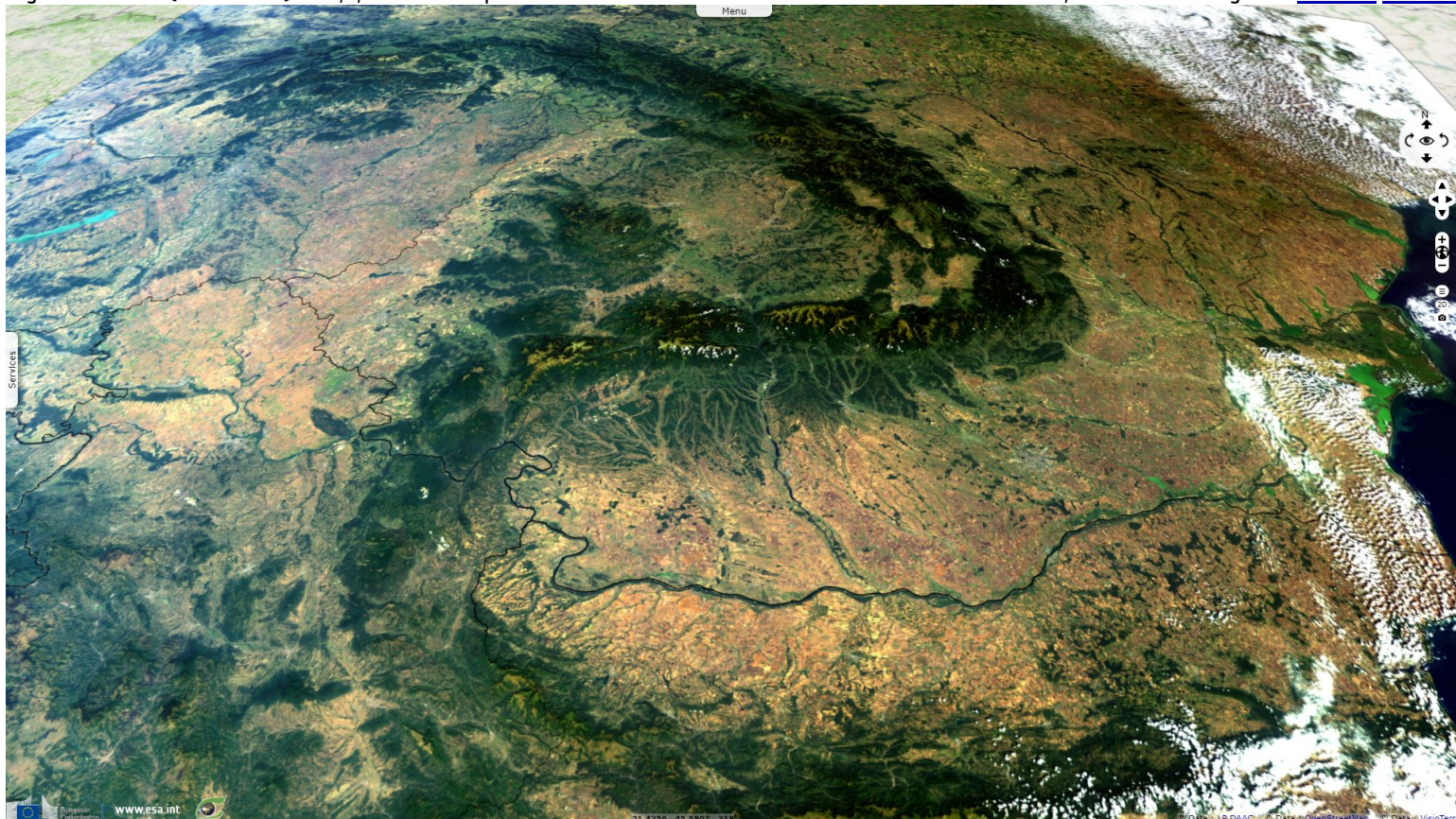
Fig. 2 - S3 OLCI (31.08.2017) - 10,6,3 colour composite - The Danube delimits the southern Romanian border, shared with Bulgaria.
