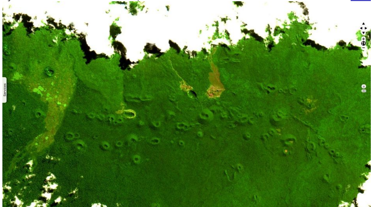
Fig. 4 - Sentinel 2A - Volcanoes on the island of Savai'i, Samoa.
