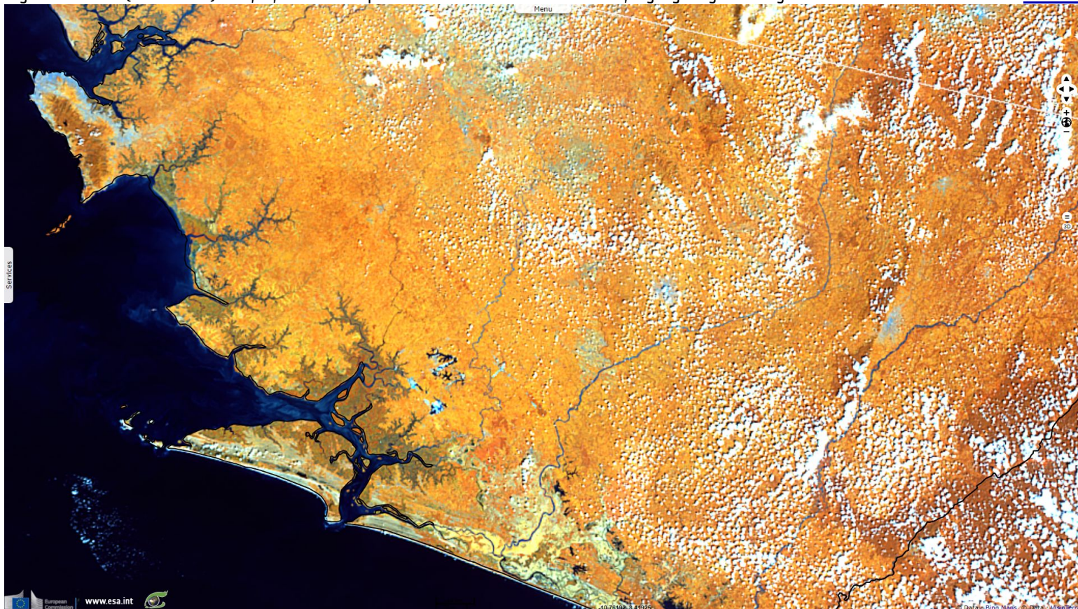
Fig. 1 - S3 OLCI (18.11.2016) - 17,11,8 colour composite - South-West of Sierra Leone, highlighting its mangroves forests.
