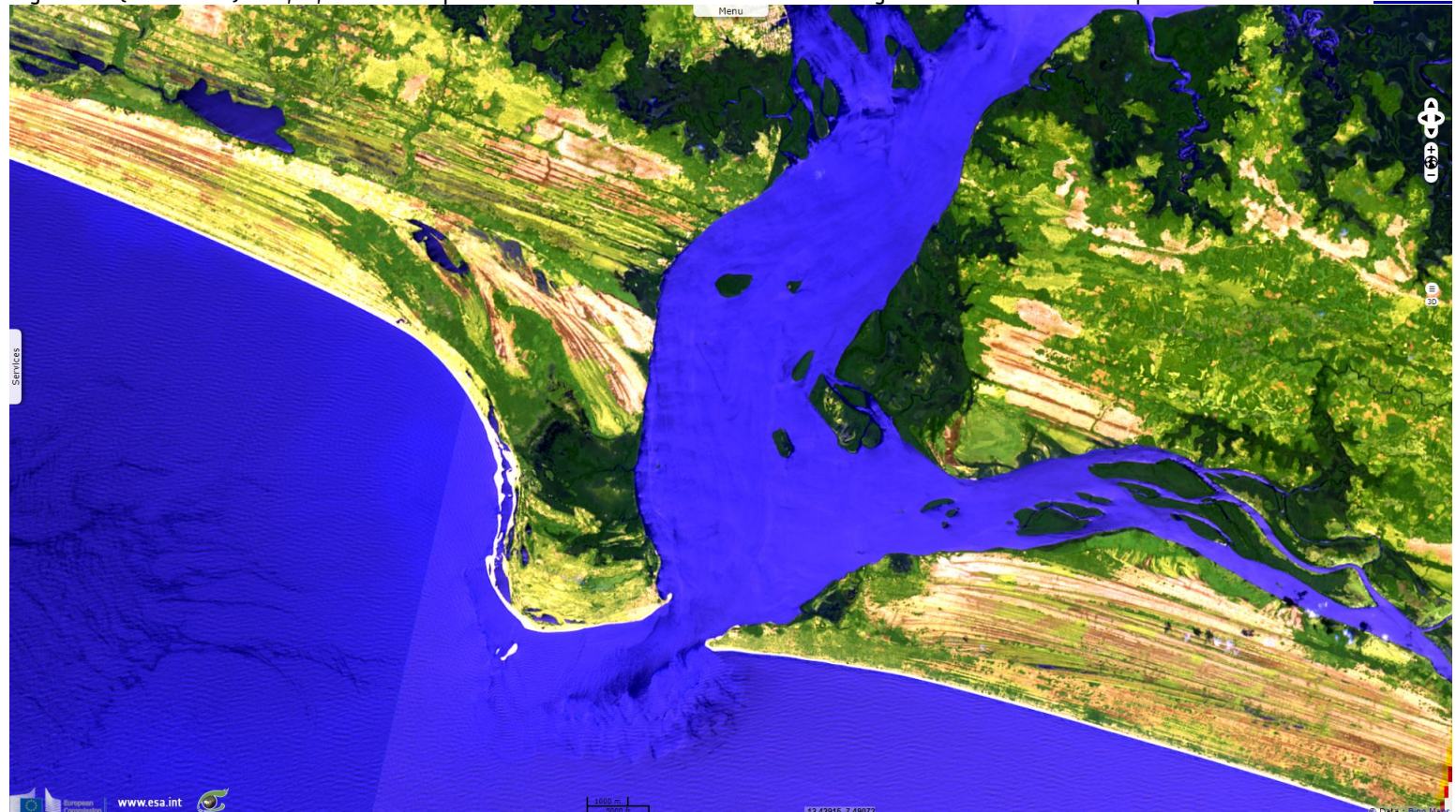
Fig. 4 - S2 (03.03.2018) - 12,11,2 colour composite - Locals & tourists benefit from its long beaches & varied landscapes. 2D view
