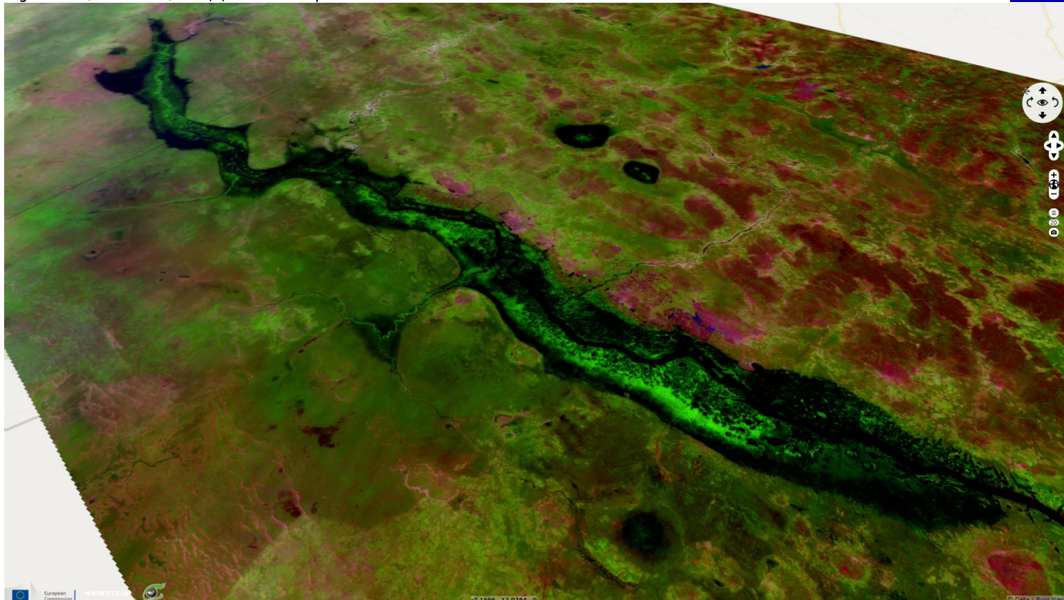
Fig. 2 - S1 (11.10.2018) - vv,vh,ndi(vh,vv) colour composite - Usually a tributary of the Black Volta, it becomes a distributary at this period.
