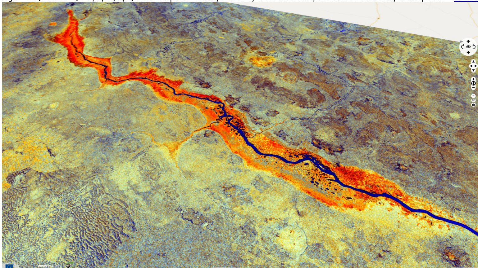
Fig. 2 - S1 (11.10.2018) - vv,vh,ndi(vh,vv) colour composite - Usually a tributary of the Black Volta, it becomes a distributary at this period.
