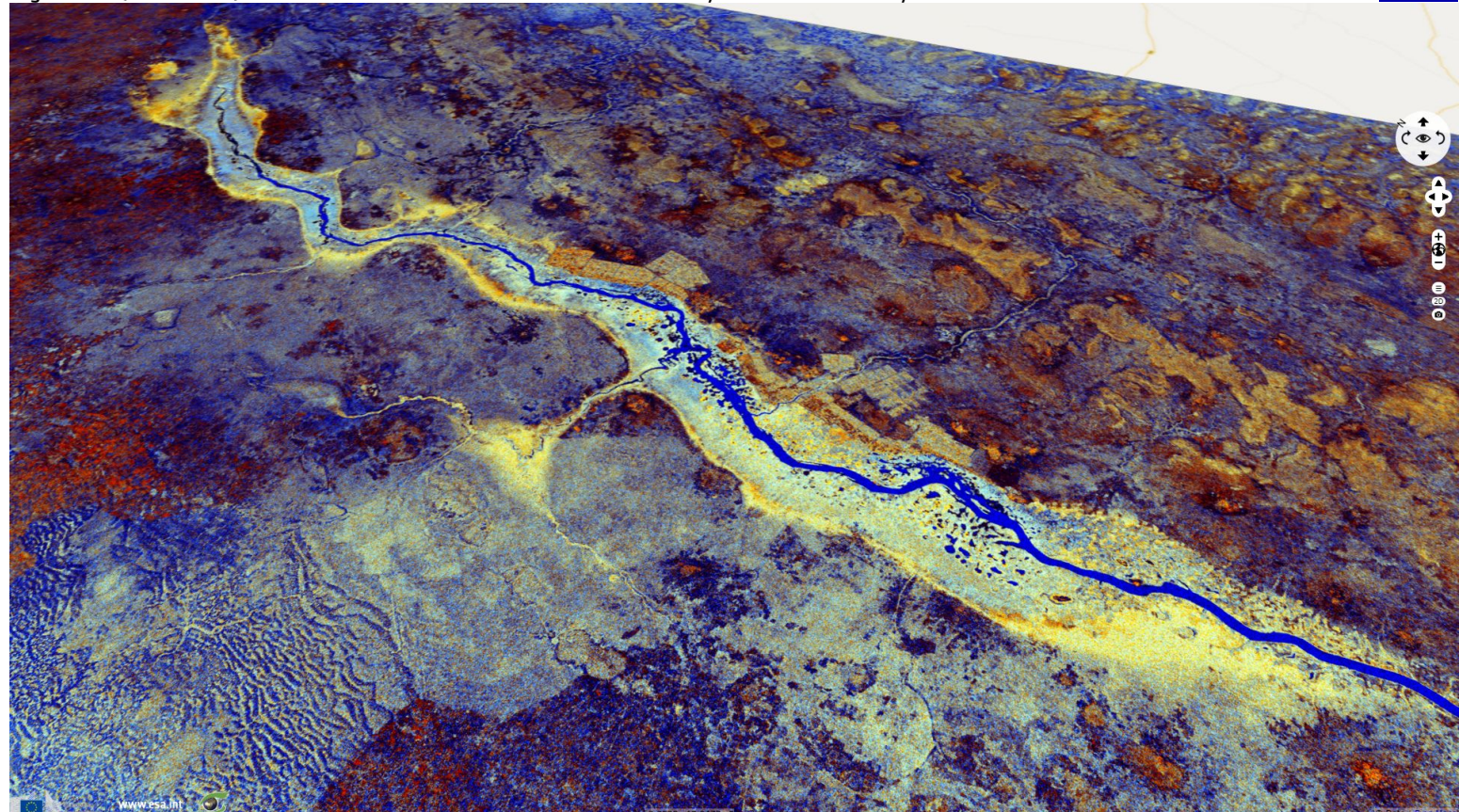
Fig. 4 - S1 (15.01.2019) - Burkina Faso & Mali declared the Sourou Valley as a Transboundary Ramsar Site the 22.01.2019.
