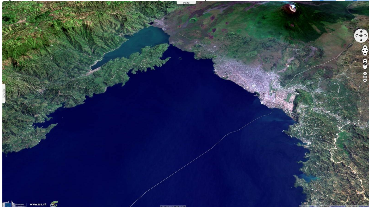
Fig.4 - Part of the Virunga, Bwindi and Volcanoes national parks, home of mountain gorilla - 8-4-3 composite
