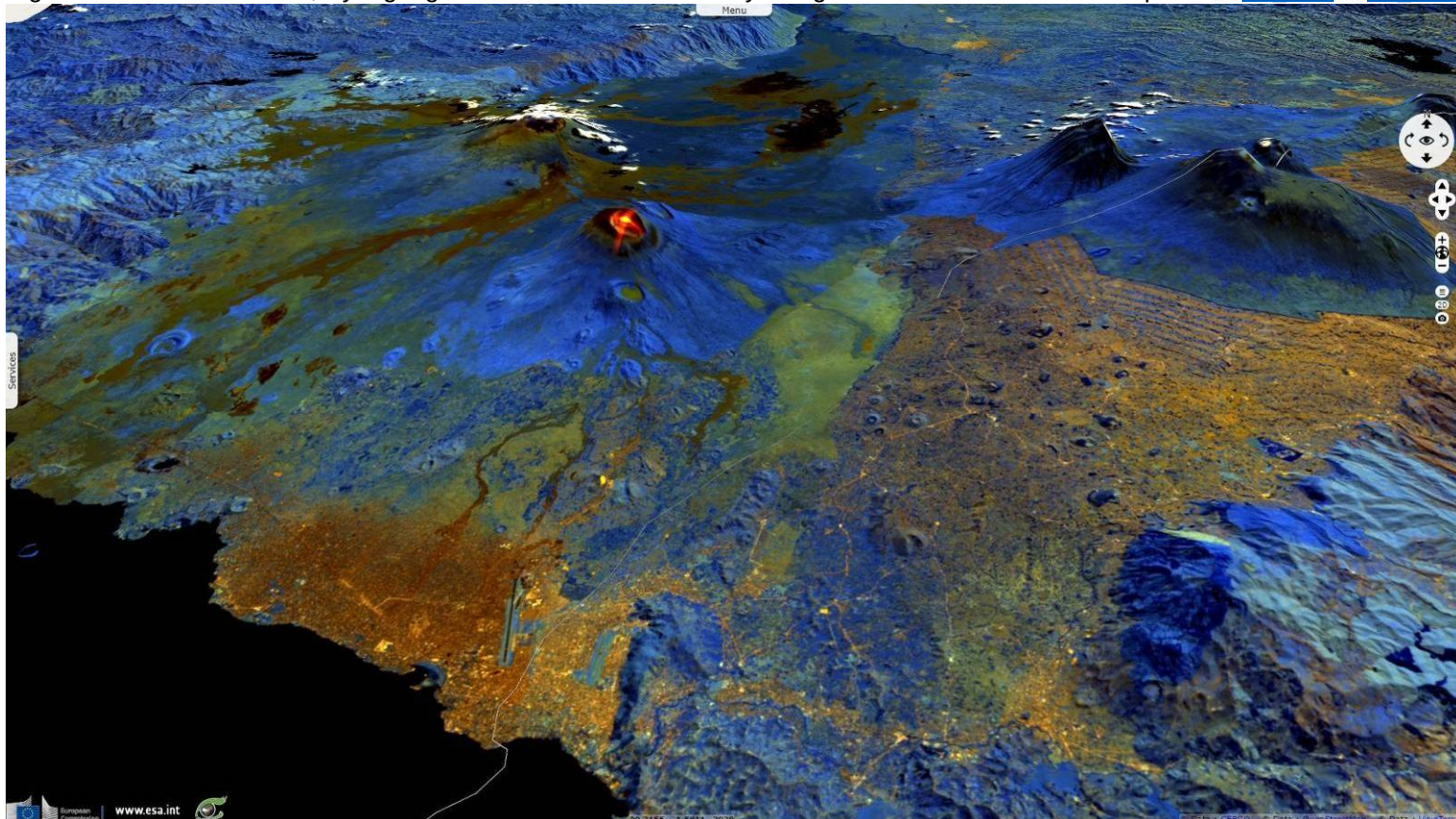
Fig. 2 - On the Albertine rift, Nyiragongo and its lava lake before Nymulagira's lava field - 12-11-8 composite 2D view 3D view
