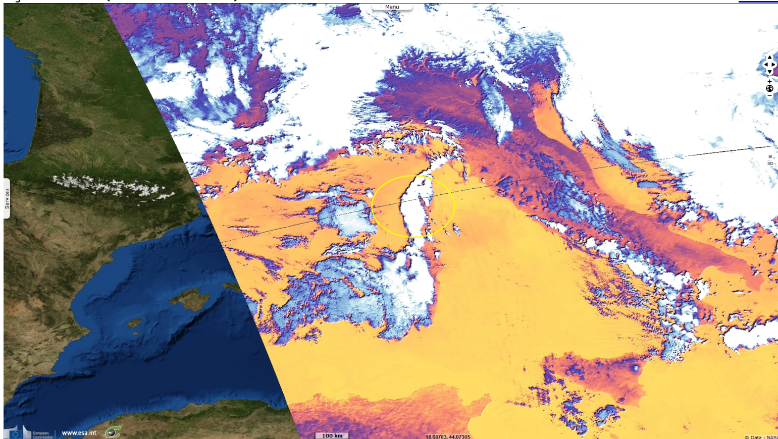
Fig. 2 - S3A SLSTR (22.12.2019 20:48/20:51) - S8 thermal band - Thermal view of the Storm Fabien over Corsica.
