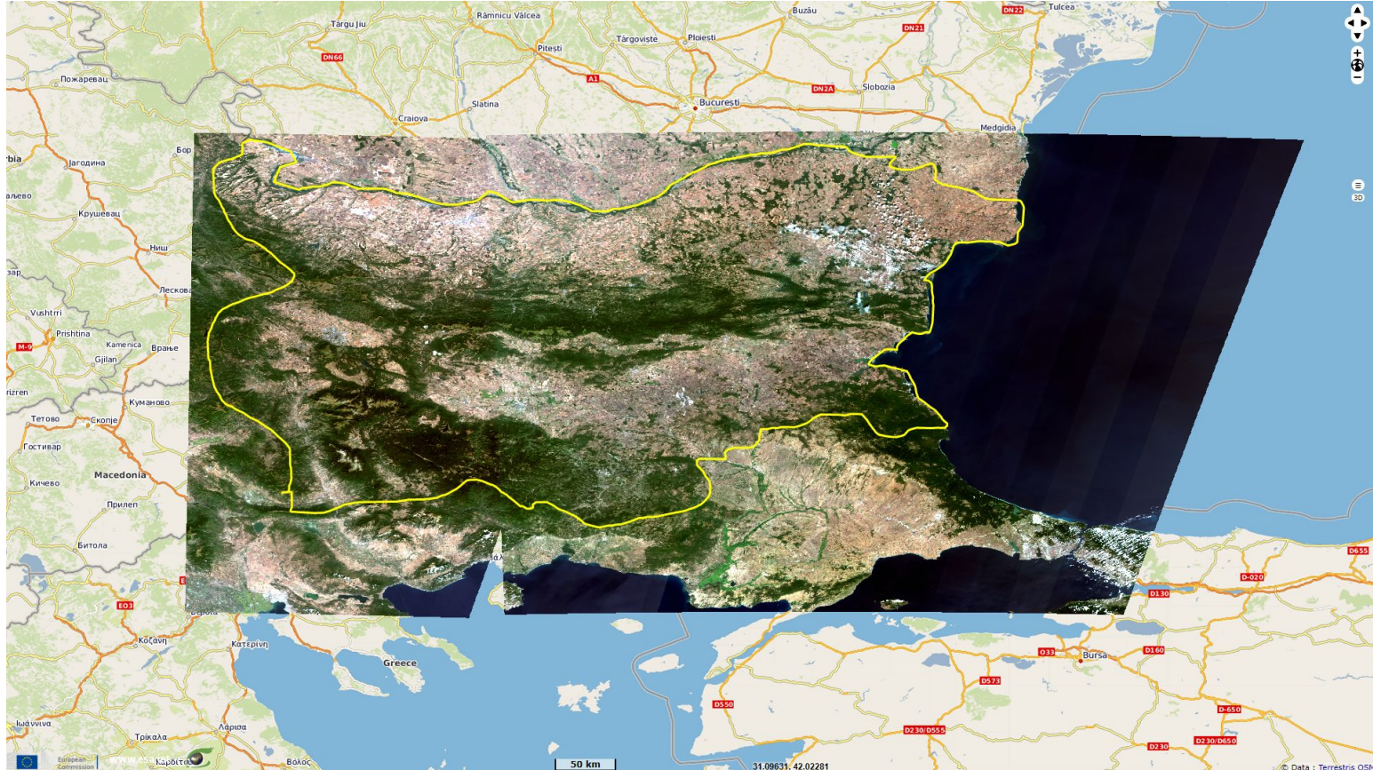
Fig. 2 - S2 (26.08.2019/29.08.2019/16.09.2019) - 11,8,2 colour composite - Full view with a colour composite that highlight the vegetation.
