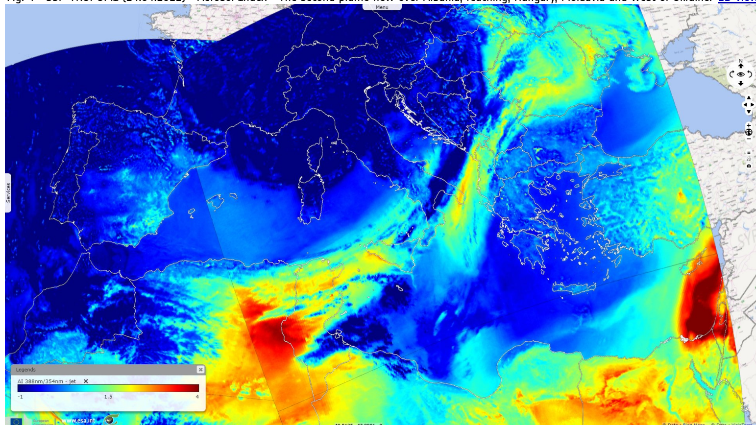
Fig. 4 - S5P TROPOMI (24.04.2022) - Aerosol Index - The second plume flew over Albania, reaching, Hungary, Moldavia and west of Ukraine. 2D view
