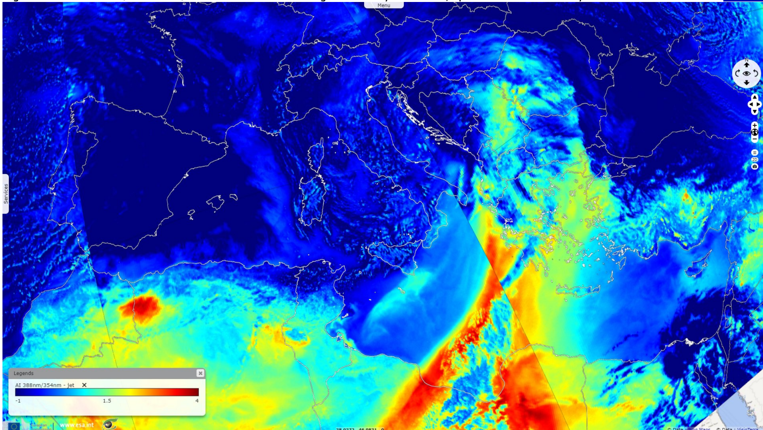
Fig. 2 - S5P TROPOMI (22.04.2022) - Aerosol Index - This tongue went beyond Greece, up to Romania and Turkey.
