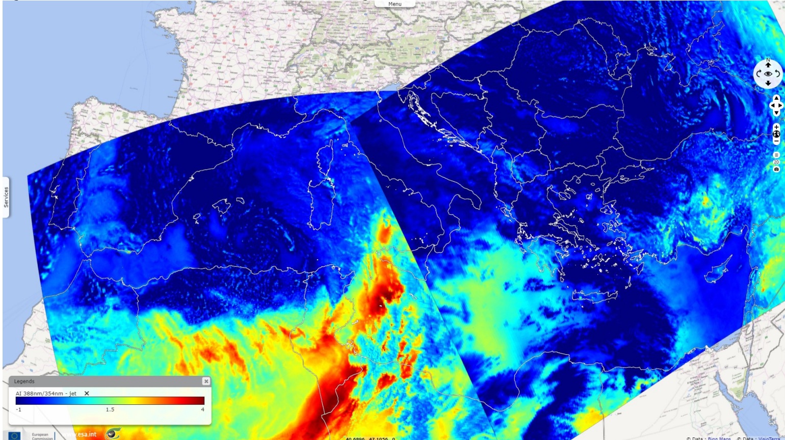
Fig. 2 - S5P TROPOMI (22.04.2022) - Aerosol Index - This tongue went beyond Greece, up to Romania and Turkey.
