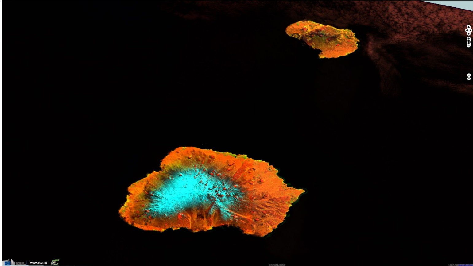
Fig. 2 - Sentinel 2A MSI (28.07.2016) on Marion Island - 11-12-4 colour composite.
