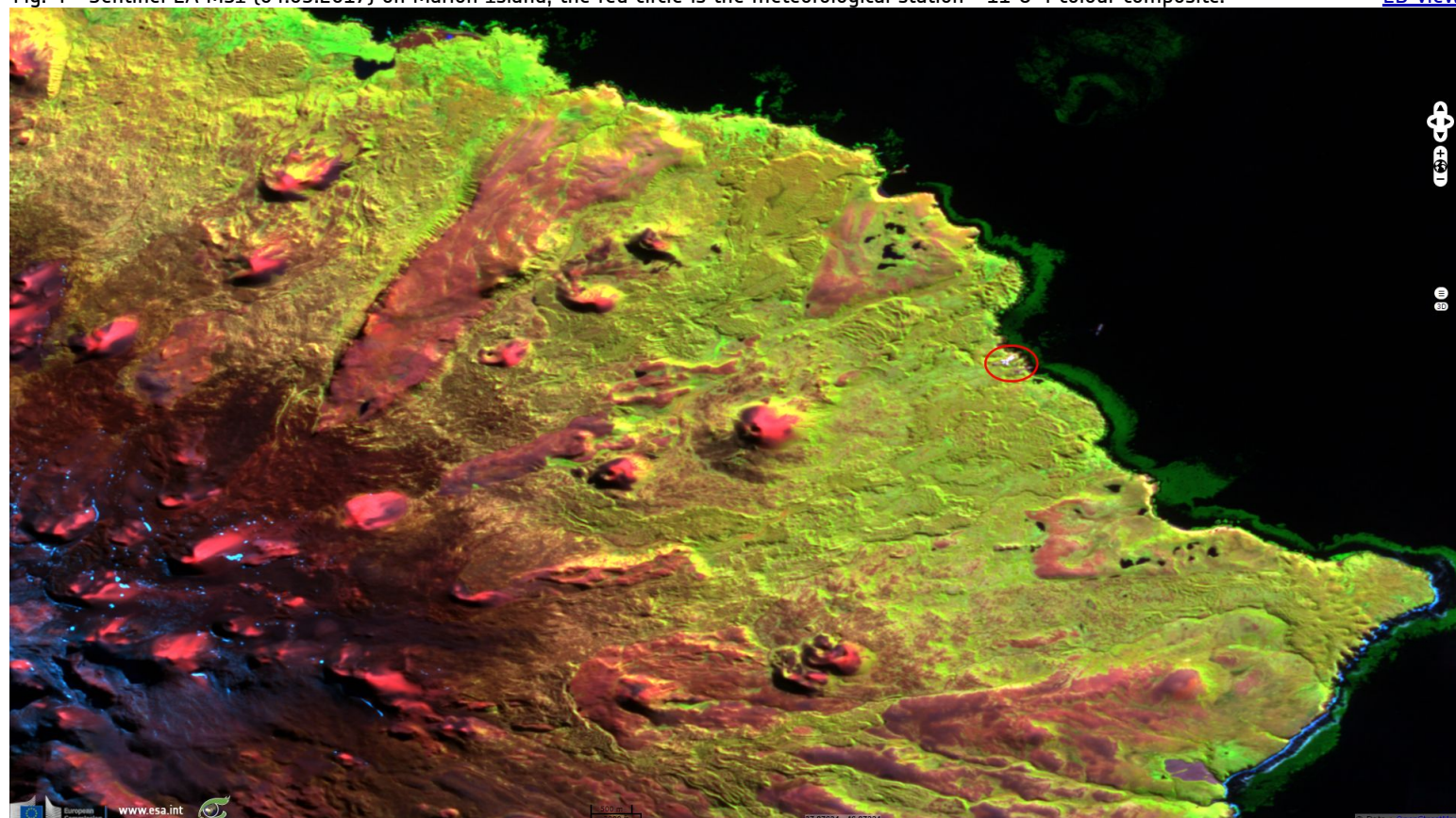
Fig. 4 - Sentinel 2A MSI (04.05.2017) on Marion Island, the red circle is the meteorological station - 11-8-4 colour composite.
