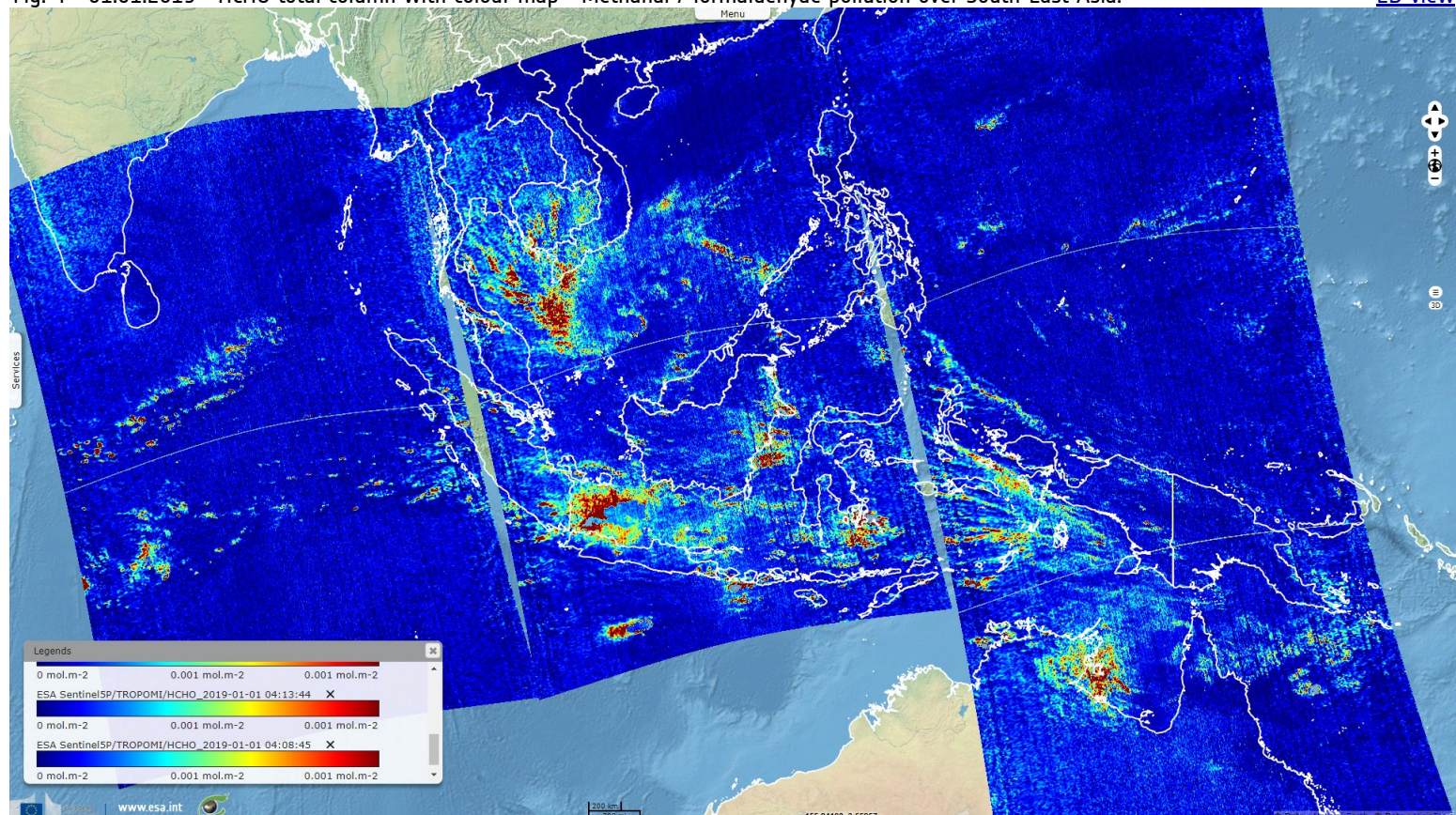
Fig. 4 - 01.01.2019 - HCHO total column with colour map - Methanal / formaldehyde pollution over South-East Asia.
