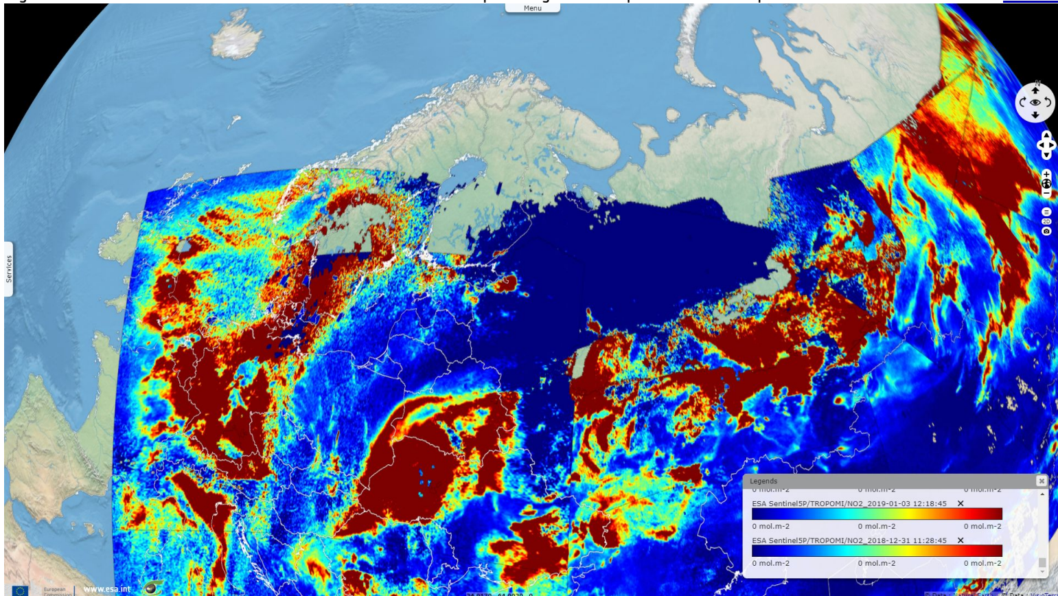
Fig. 2 - 31.12.2018 - 01.01.2019 - NO2 total column with colour map - Nitrogen dioxide pollution over Europe & Russia
