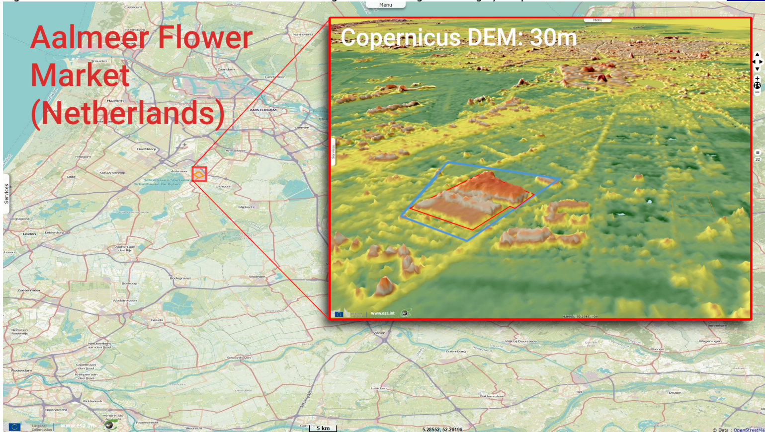
Fig. 1 - COP-DEM/GLO-30 - The Aalsmeer Flower Auction building is the tenth largest building by footprint in the world.
