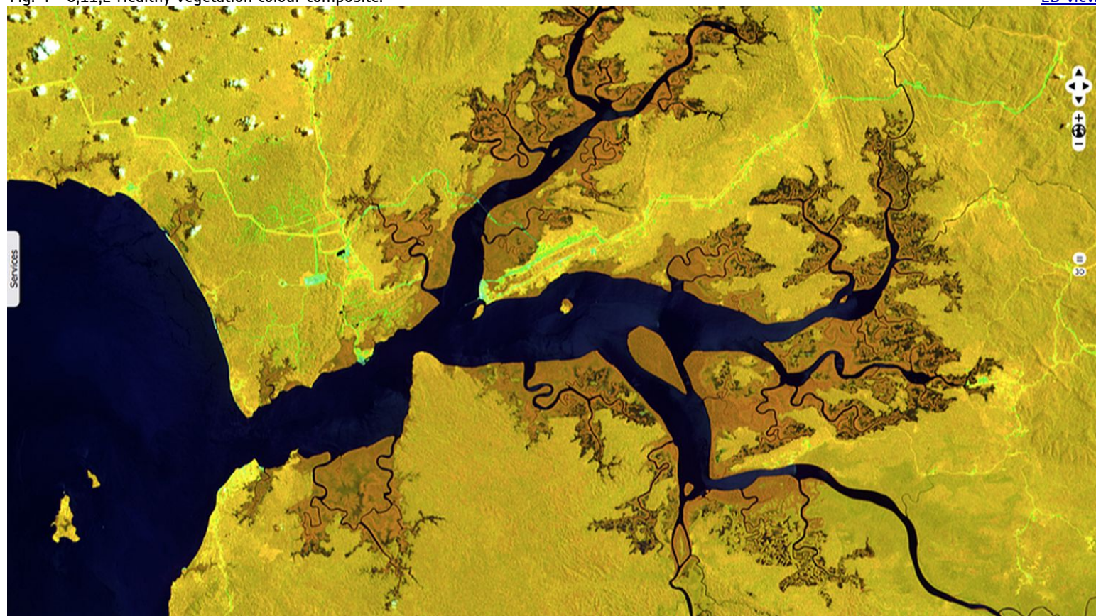
Fig. 4 - 8,11,2 Healthy vegetation colour composite.
