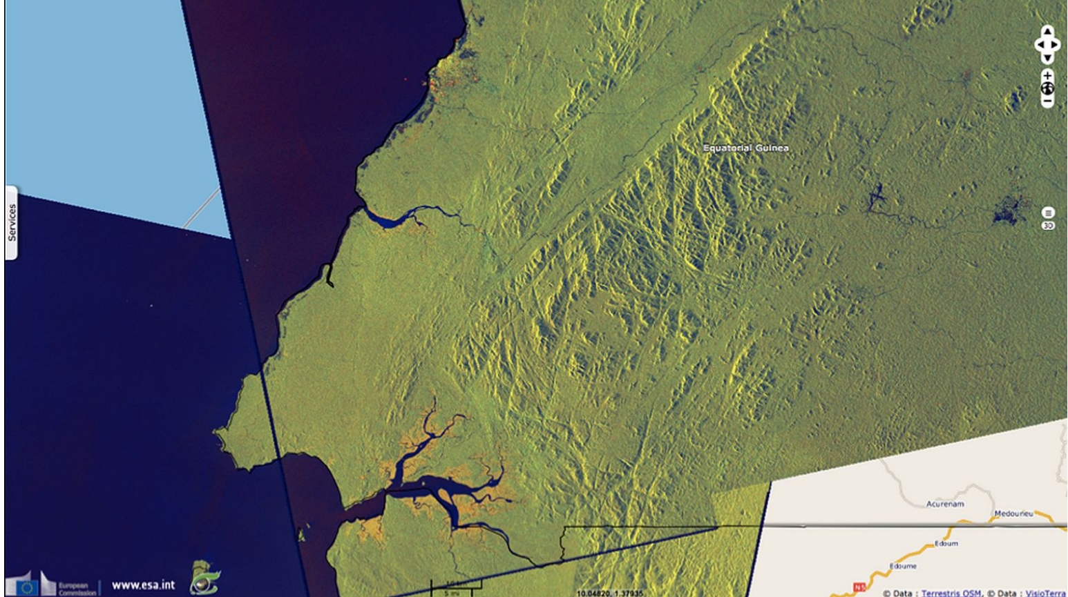
Fig. 2 - Sentinel 2A (02.05.2017) - 11,8,2 Agriculture composite - City of Bata, economic capital of Equatorial Guinea.
