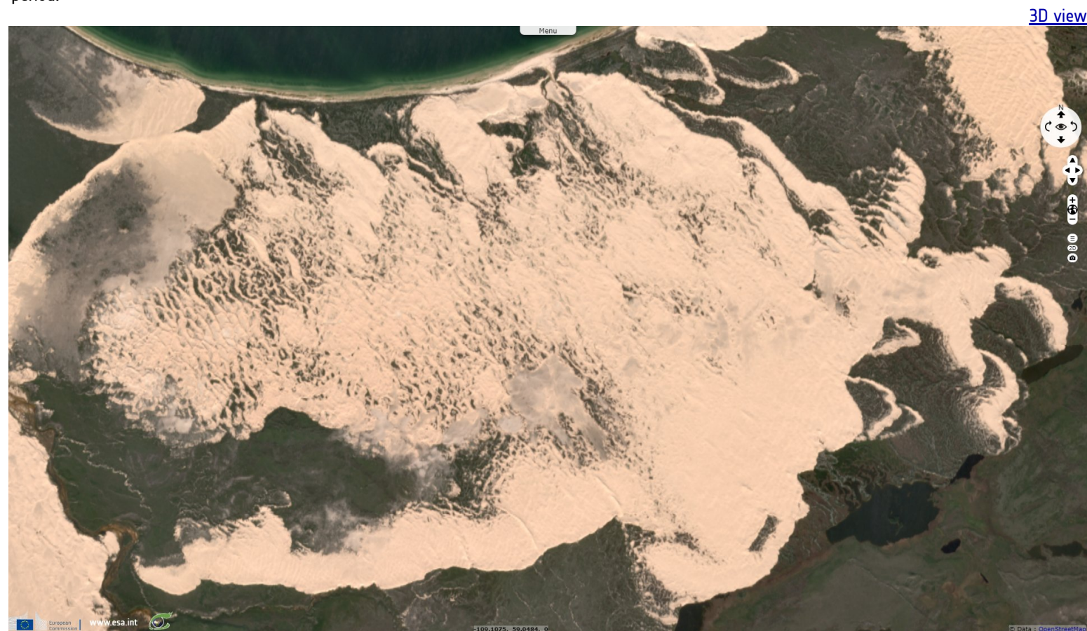
Fig. 3 - S2 (23.09.2023) - Zoom on one of the dune areas. The Athabasca Sand Dunes formed from local sandstone near the end of the last glacial period.
