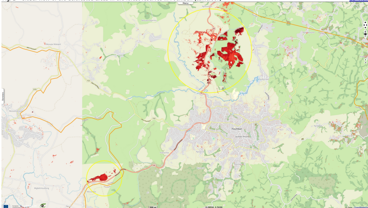
Fig. 2 - Global view of the deforested areas in the forest reserves in Fouban (Cameroon)
