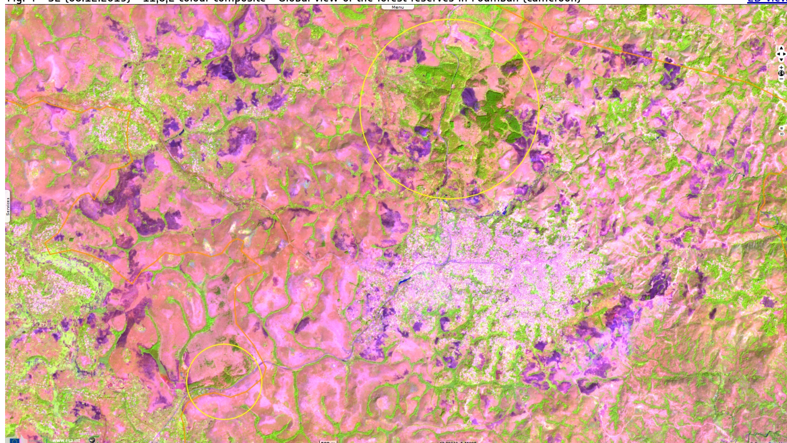
Fig. 4 - S2 (08.12.2019) - 11,8,2 colour composite - Global view of the forest reserves in Fouban (Cameroon)
