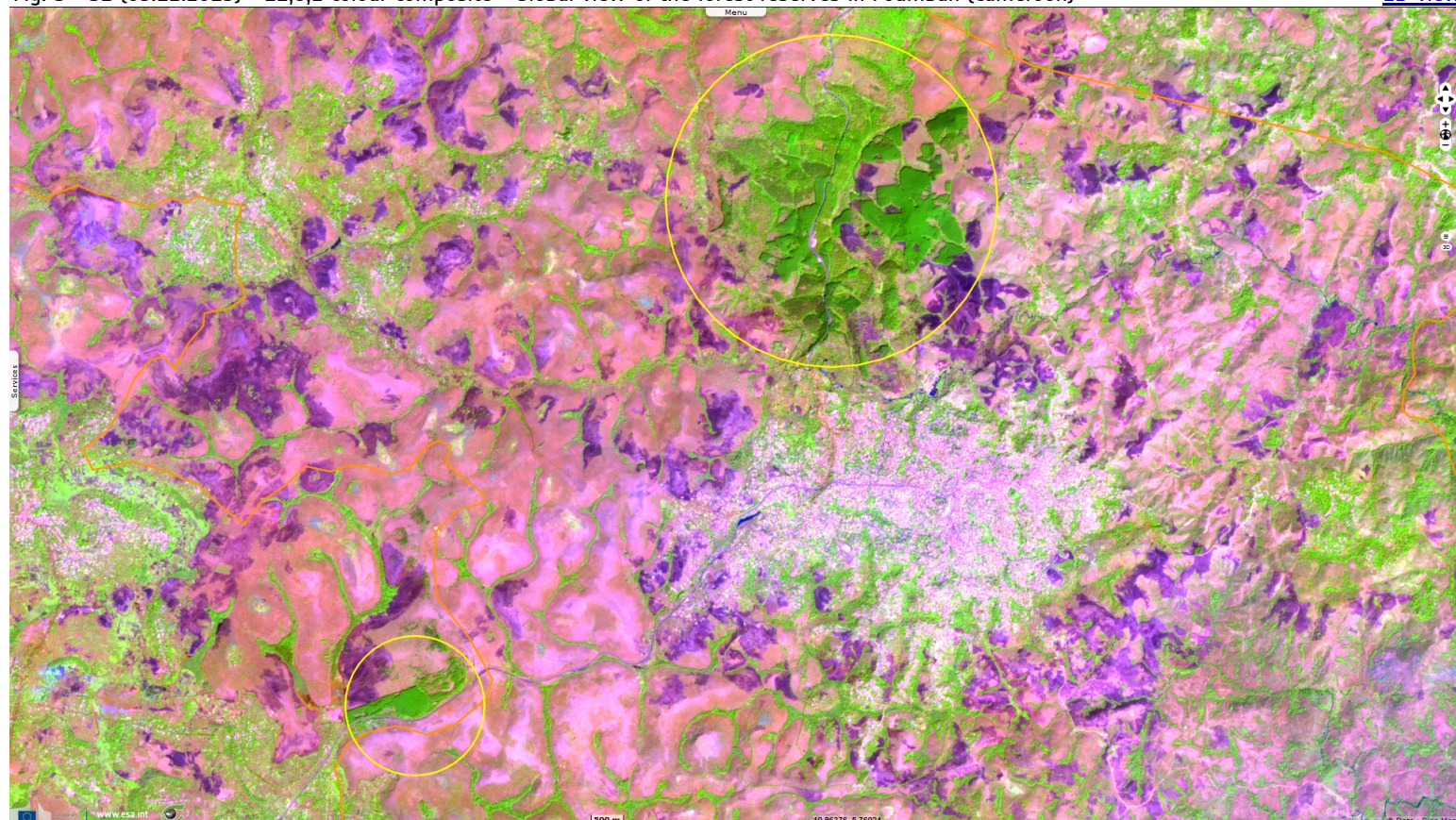
Fig. 4 - S2 (08.12.2019) - 11,8,2 colour composite - Global view of the forest reserves in Fouban (Cameroon)
