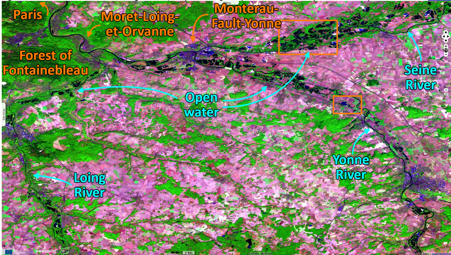
Fig. 1 - S2 (17.09.2020) - Often located along riverbeds, many sand and gravel quarries are subsequently renaturalized as ponds.
