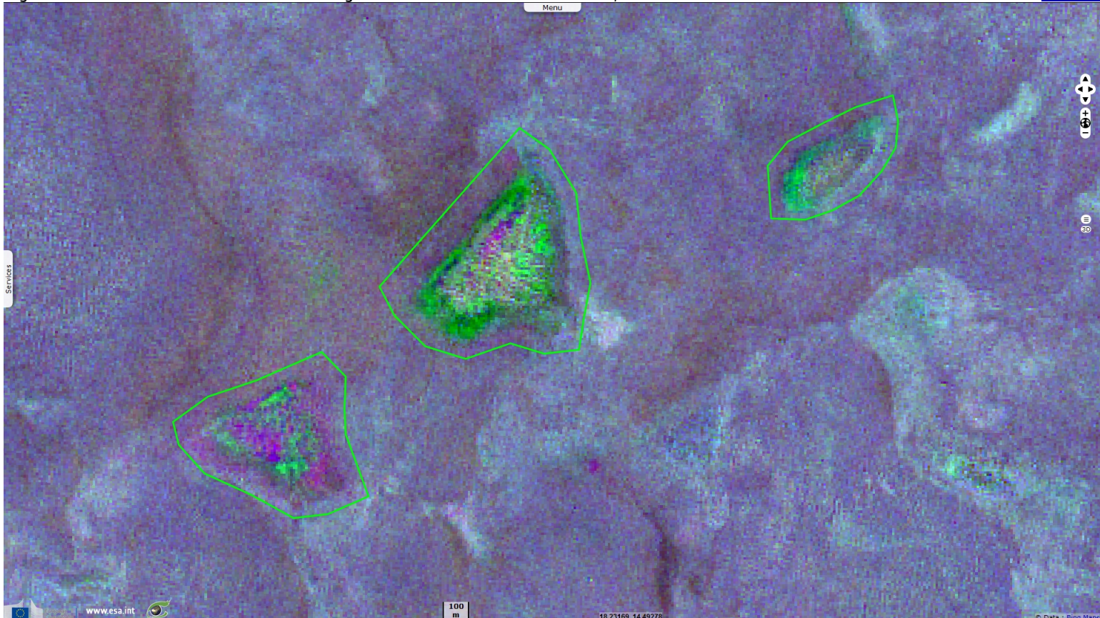
Fig. 2 - Difference between the Sentinel-2 images observed on November 17 and 7, 2019.
