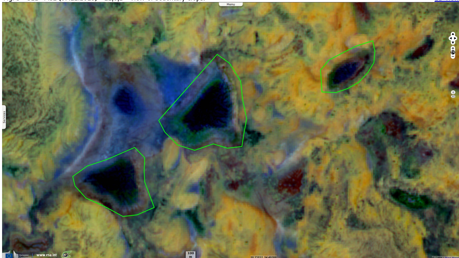
Fig. 4 - S2B- MSI (17.11.2019) - 11,8,2 - View of sedentary crops 10 days latter.
