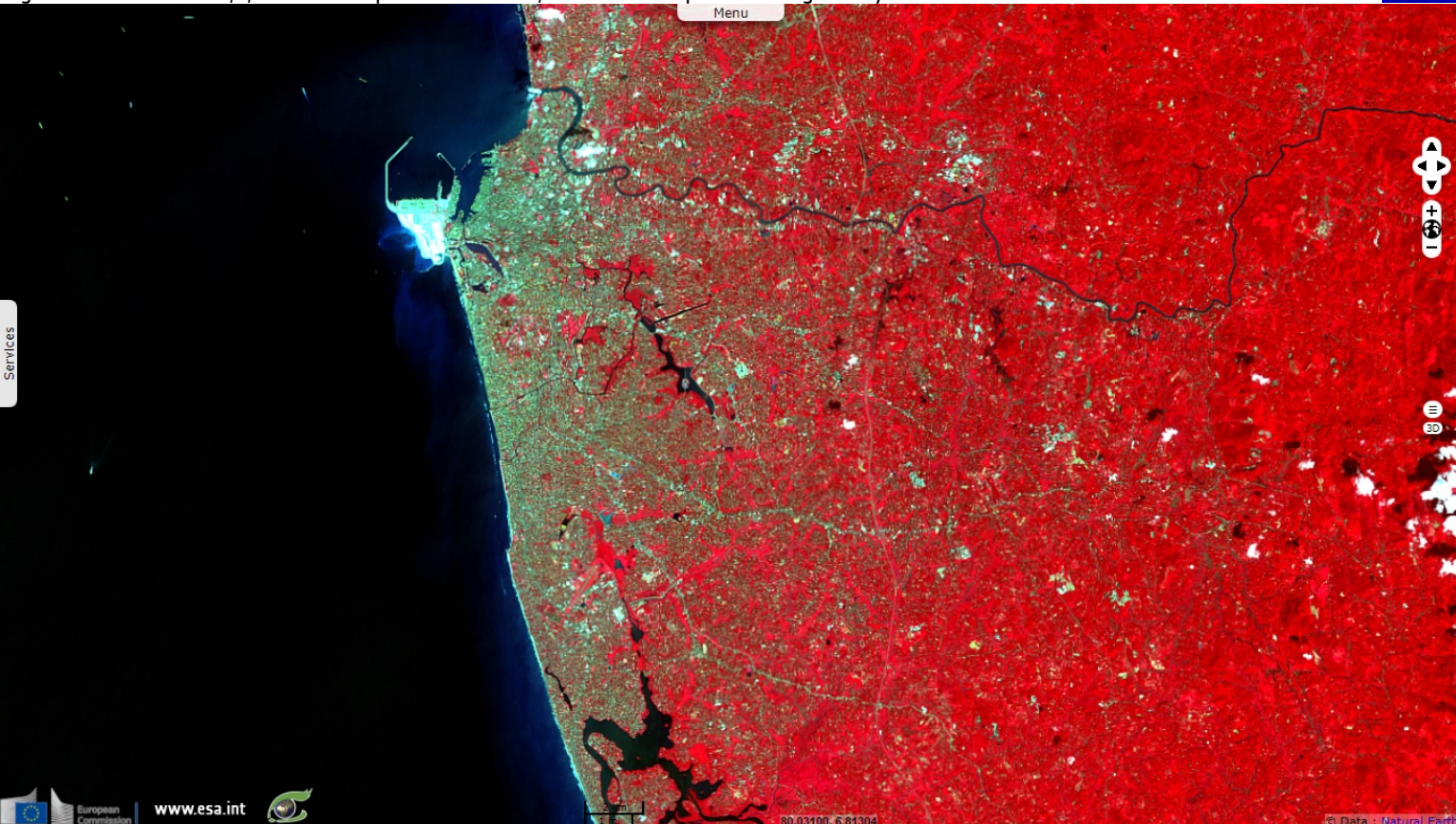
Fig. 2 - 2017-12-07 - 8,4,3 colour composite - Colombo, commercial capital and largest city of Sri Lanka.
