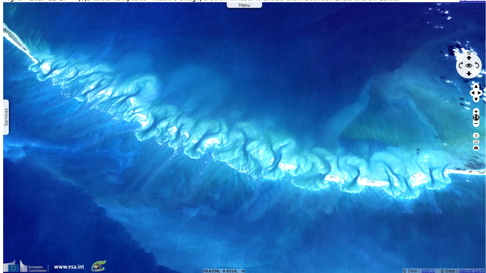
Fig. 4 - 2017-11-17 - 4,3,2 colour composite - Lagoons of the Northern Province of Sri Lanka.
