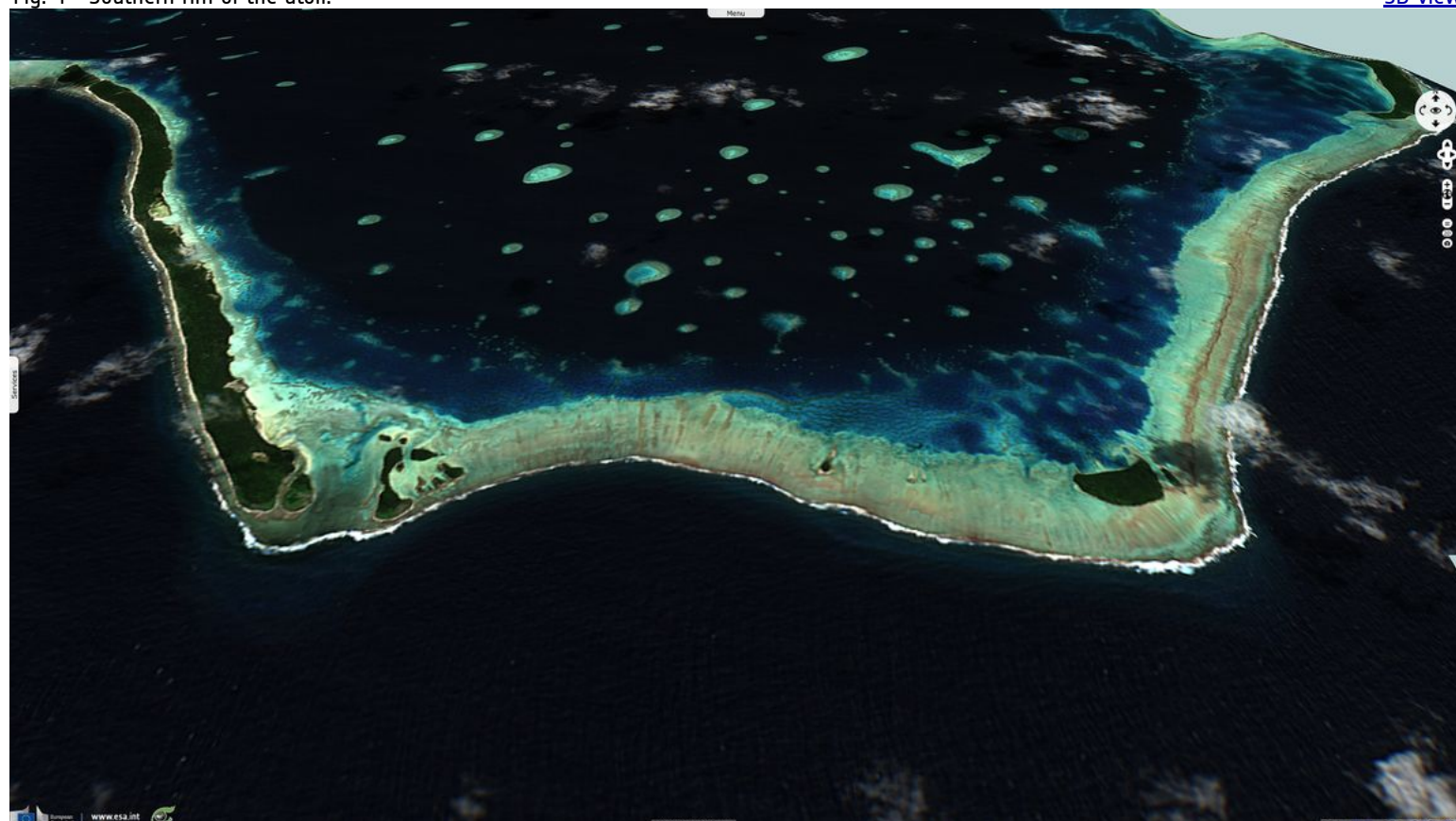
Fig. 4 - Southern rim of the atoll.
