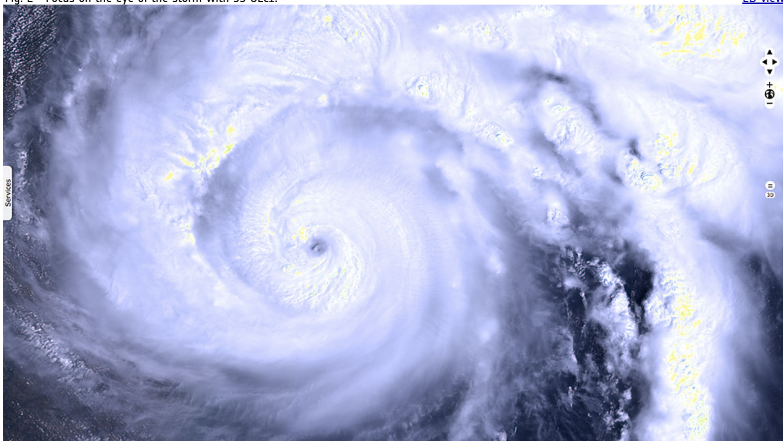
Fig. 2 - Focus on the eye of the storm with S3 OLCI.
