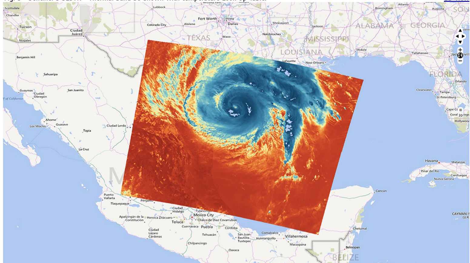
Fig. 3 - Sentinel 3 SLSTR - Thermal band S8 shown with temperature Look Up Table.
