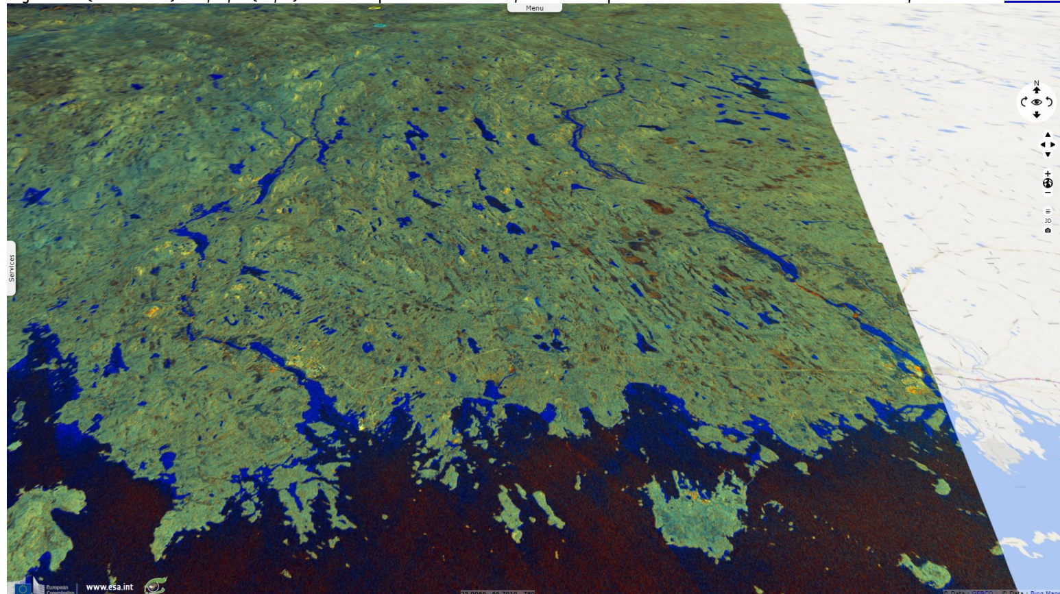
Fig. 4 - S1 (04.10.2018) - vv,vh,ndi(vh,vv) colour composite - For 200 km, both follow parallel courses that end in Gulf of Bothnia, Baltic Sea.
