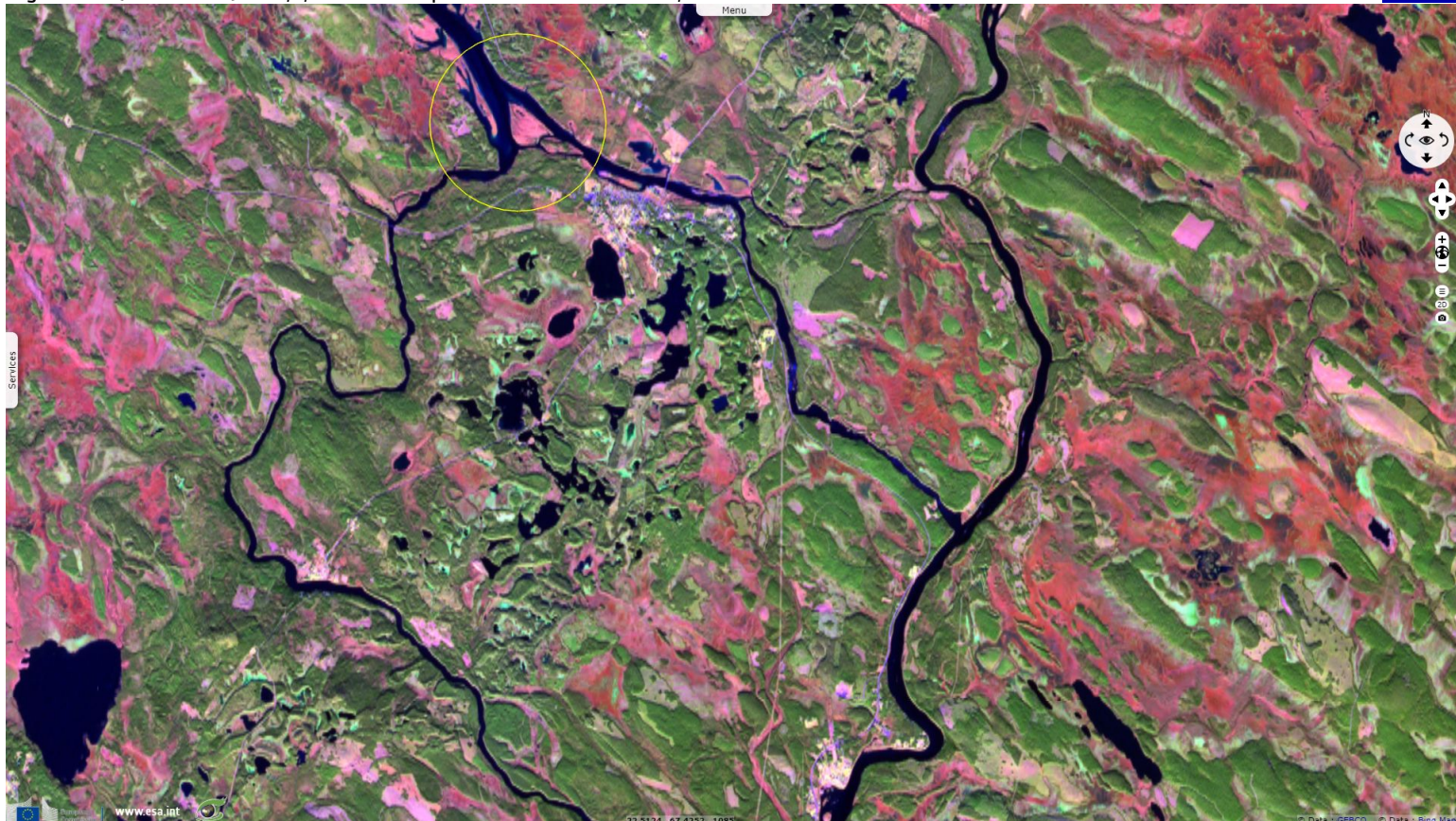
Fig. 2 - S1 (02.10.2018) - vv,vh,vv colour composite - 52 km long, Tärendö River bifurcation is the second longest in the world.. 3D view
