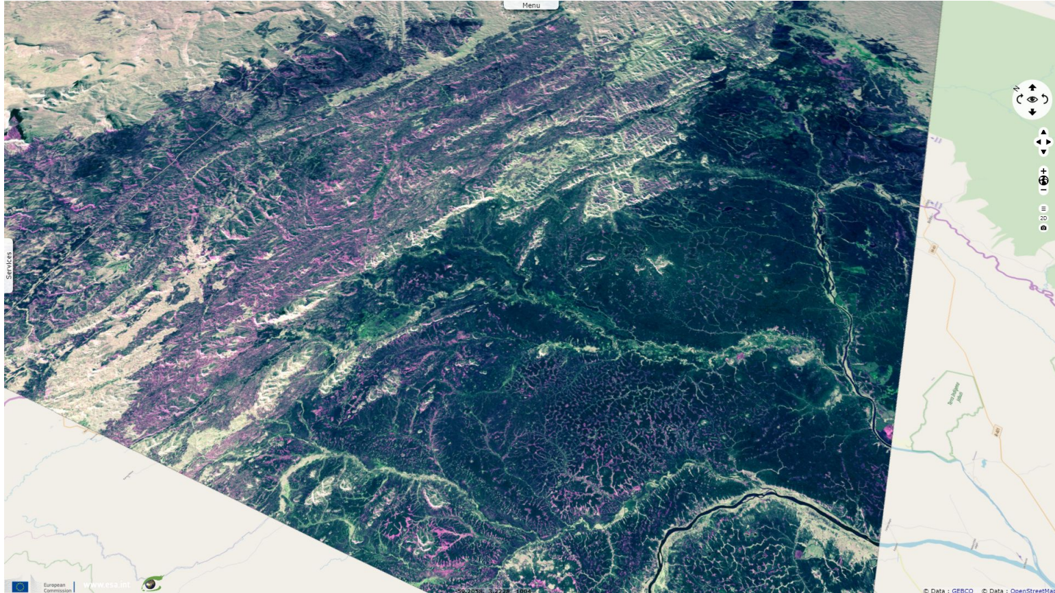
Fig. 2 - S2 (18.11.2018) - 11,8,2 colour composite - In 2005, it became a 17000km 2 reserve where live 17000 indigenous people.
