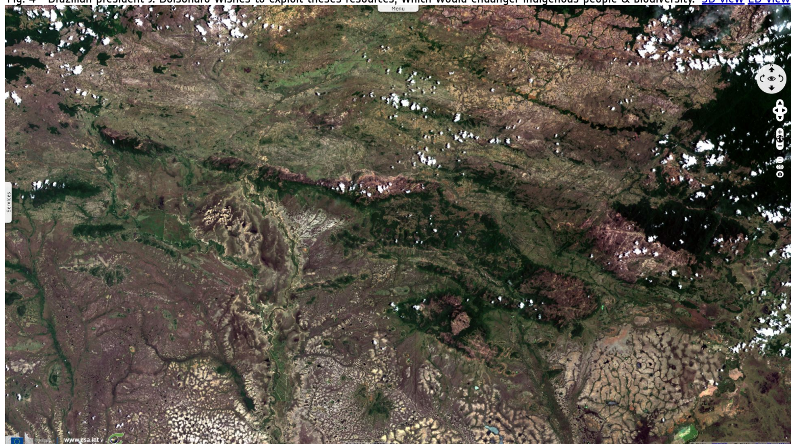
Fig. 4 - Brazilian president J. Bolsonaro wishes to exploit these resources, which would endanger indigenous people & biodiversity. 3D view 2D view
