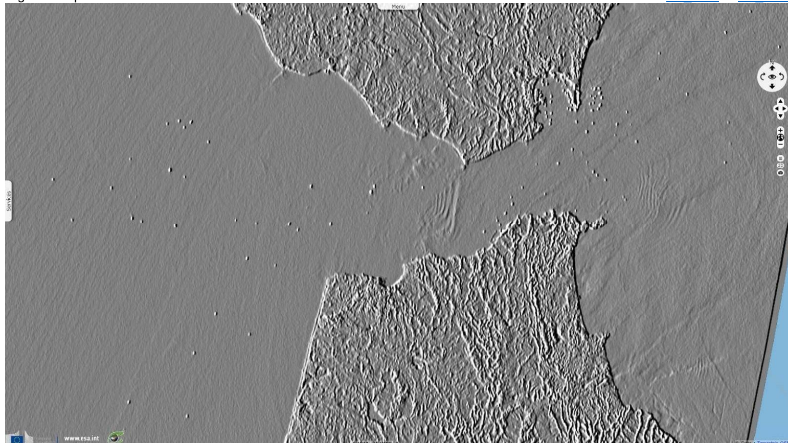
Fig. 2 - VV polarisation with “3x3 Gradient W-E” convolution.
